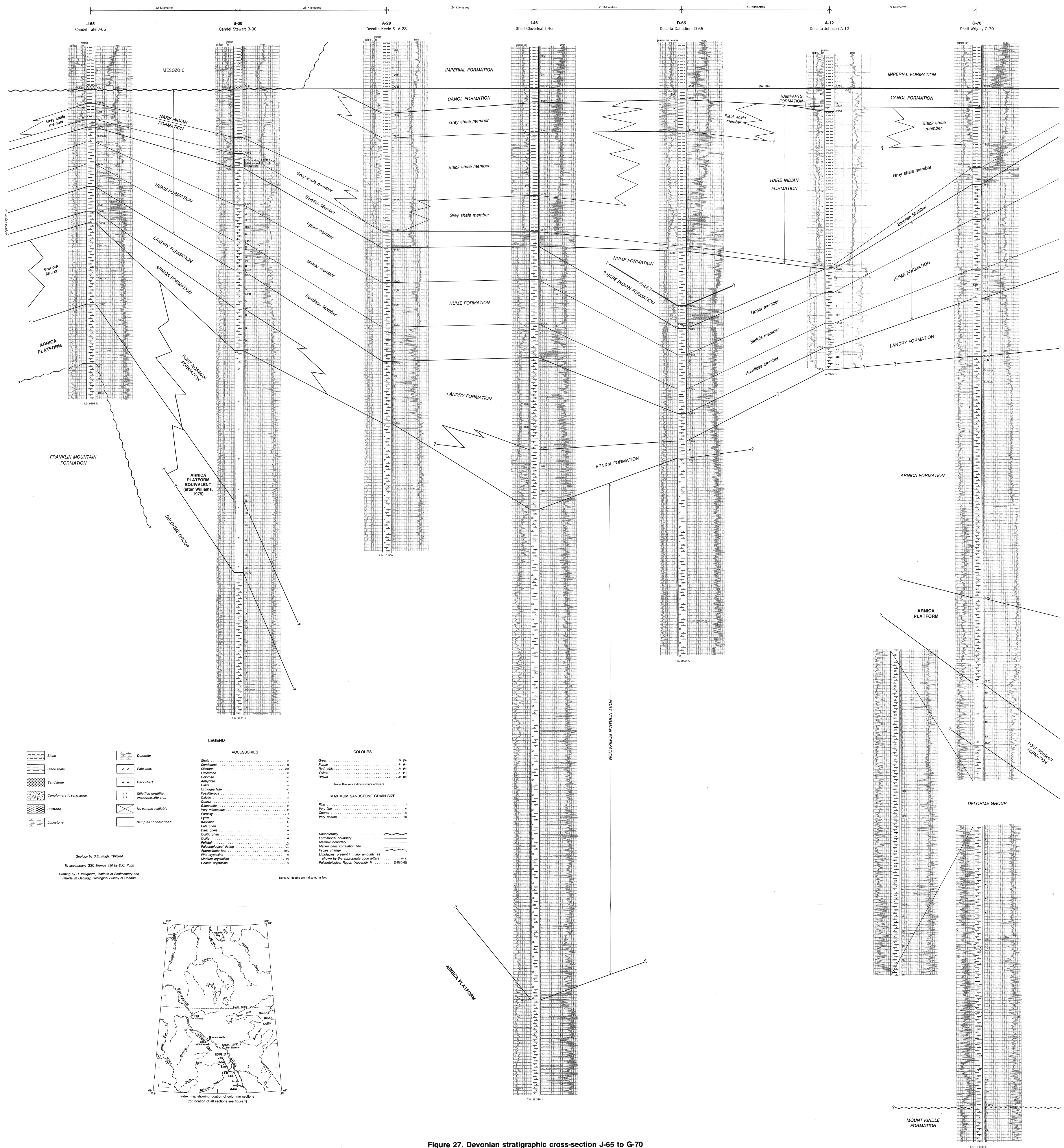
Figure 27. Devonian stratigraphic cross-section J-65 to G-70
