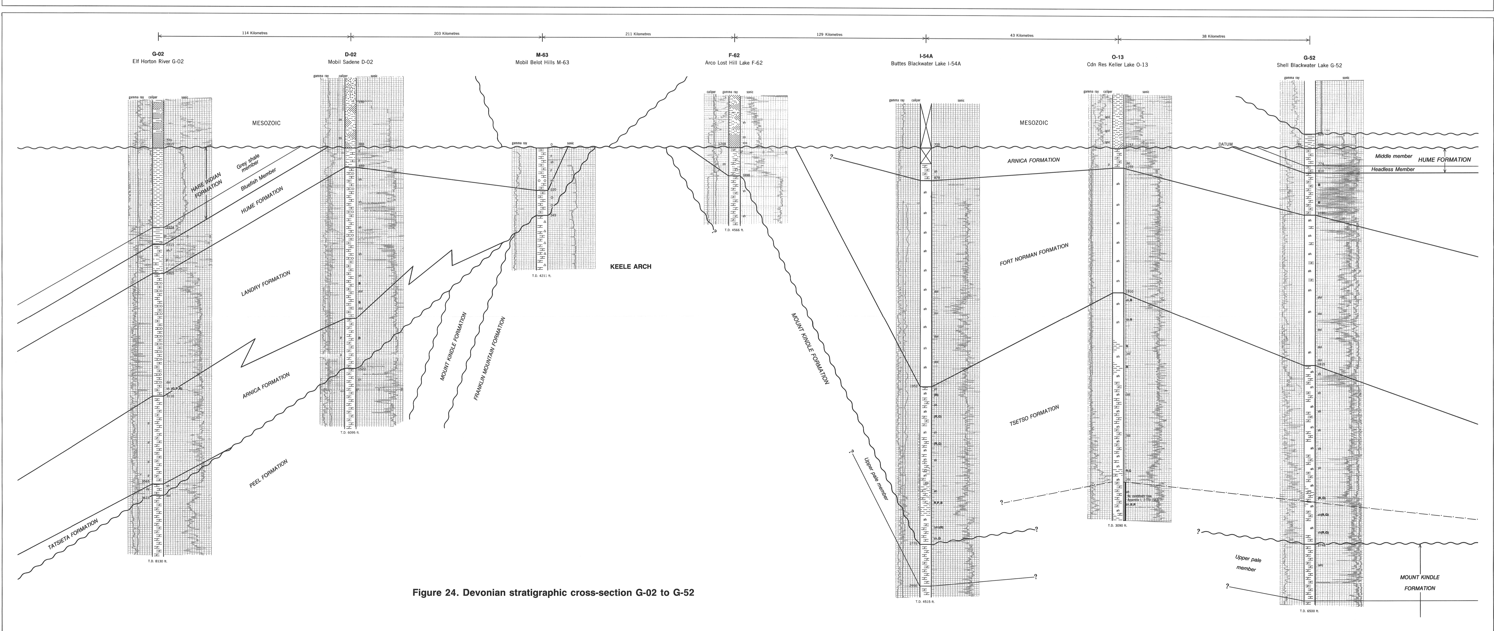
Figure 23. Ronning Group stratigraphic cross-section I-01 to F-62
