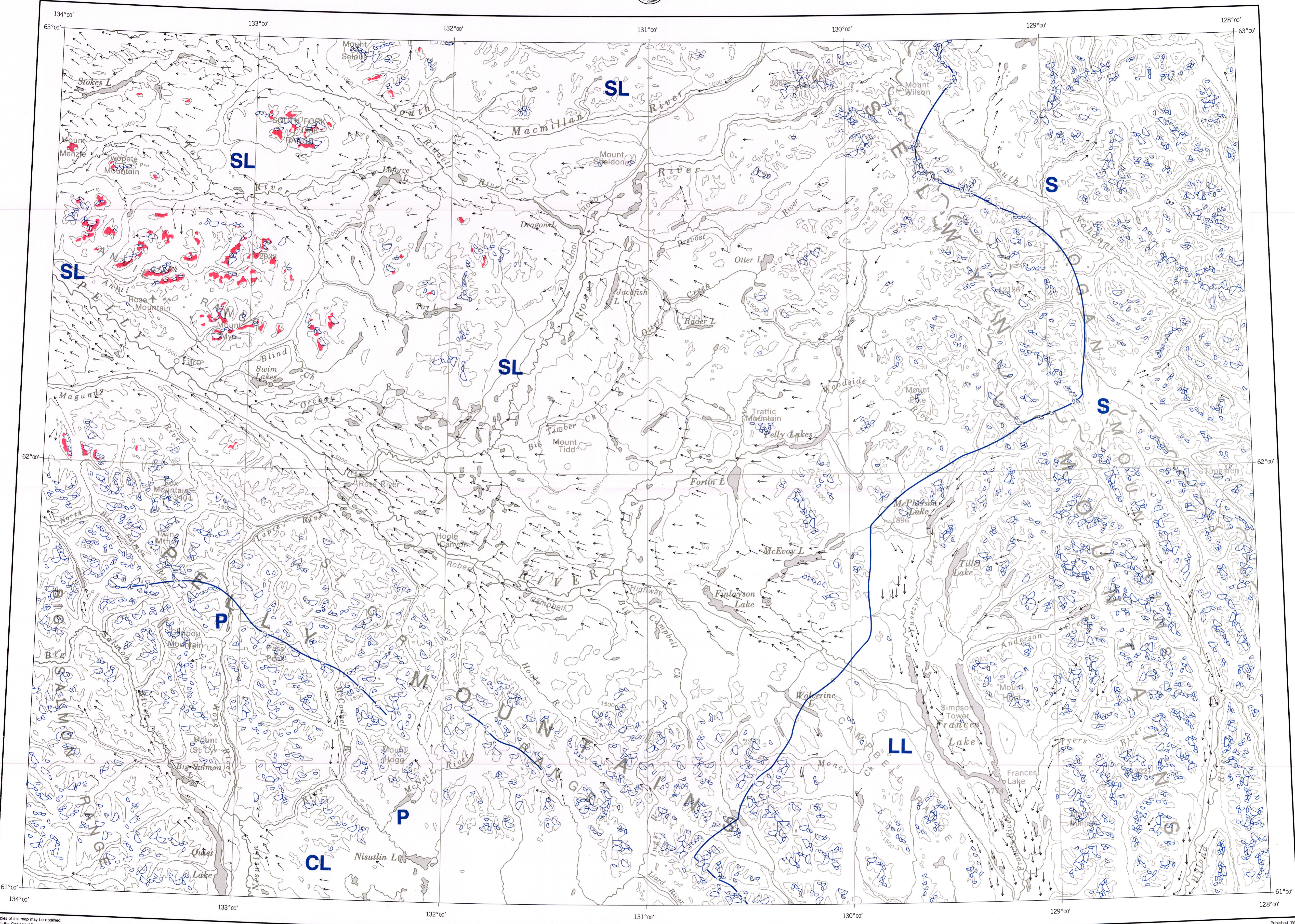
Figure 30. Ice-flow and ice-source areas
