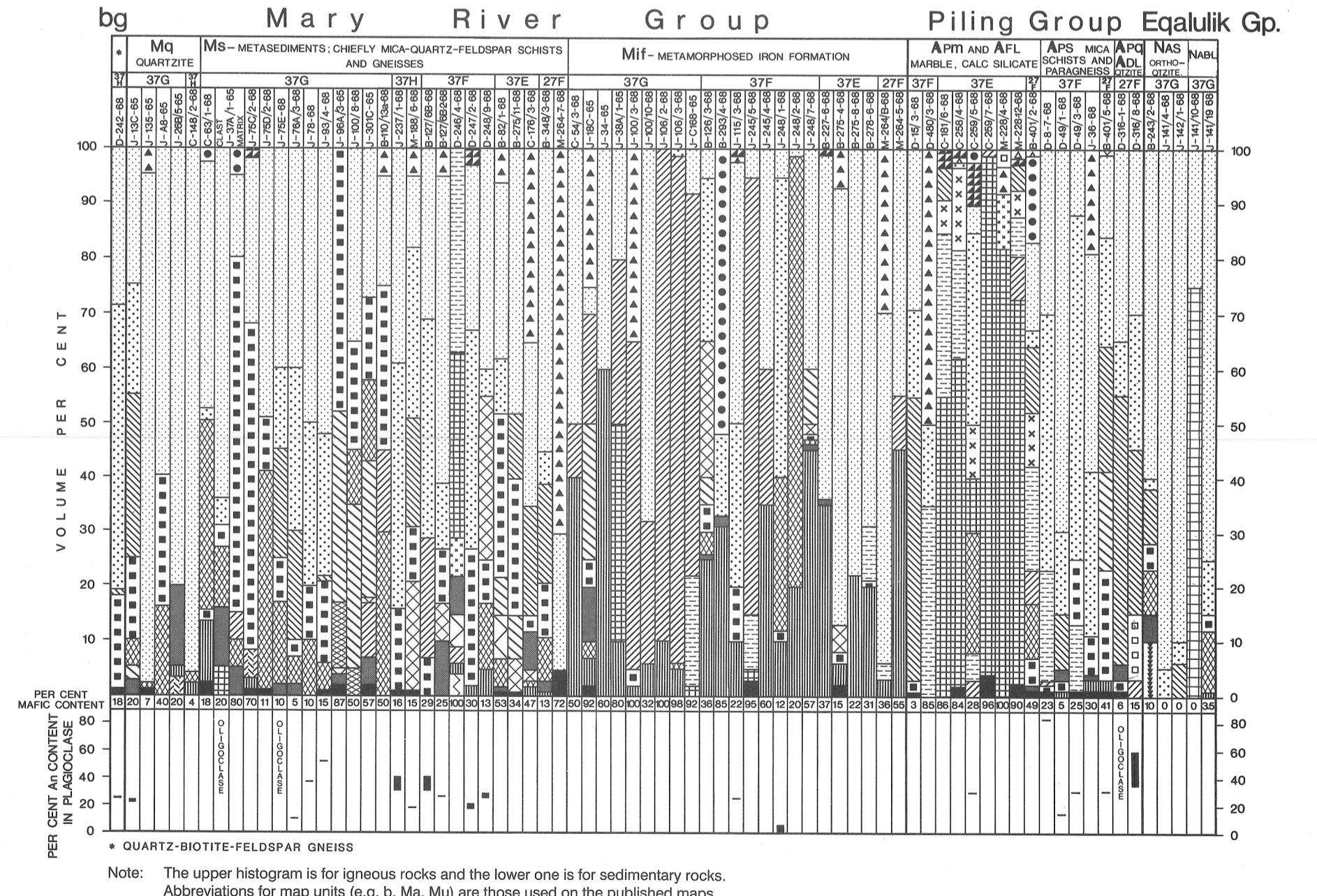
Figure 29. Mineral composition histograms for the Mary River, Piling, and Eequaluk groups, and for map units b (metamorphosed diabase), bg (paragneiss), and Hg (Franklin and Borden diabases)
