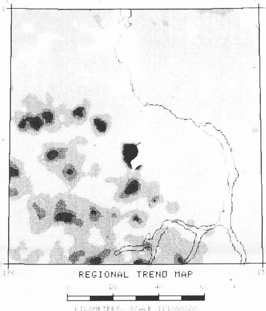
The regional geochemical trend map displayed above utilized a moving weighted average using an inverse distance function (1/d 3 ) to filter out minor irregularities and emphasize broad-scale regional features. Single point anomalies may be suppressed or eliminated, however, geological units which are chemically enriched, or large metallic deposits undergoing weathering would be expected to produce identifiable anomalies
