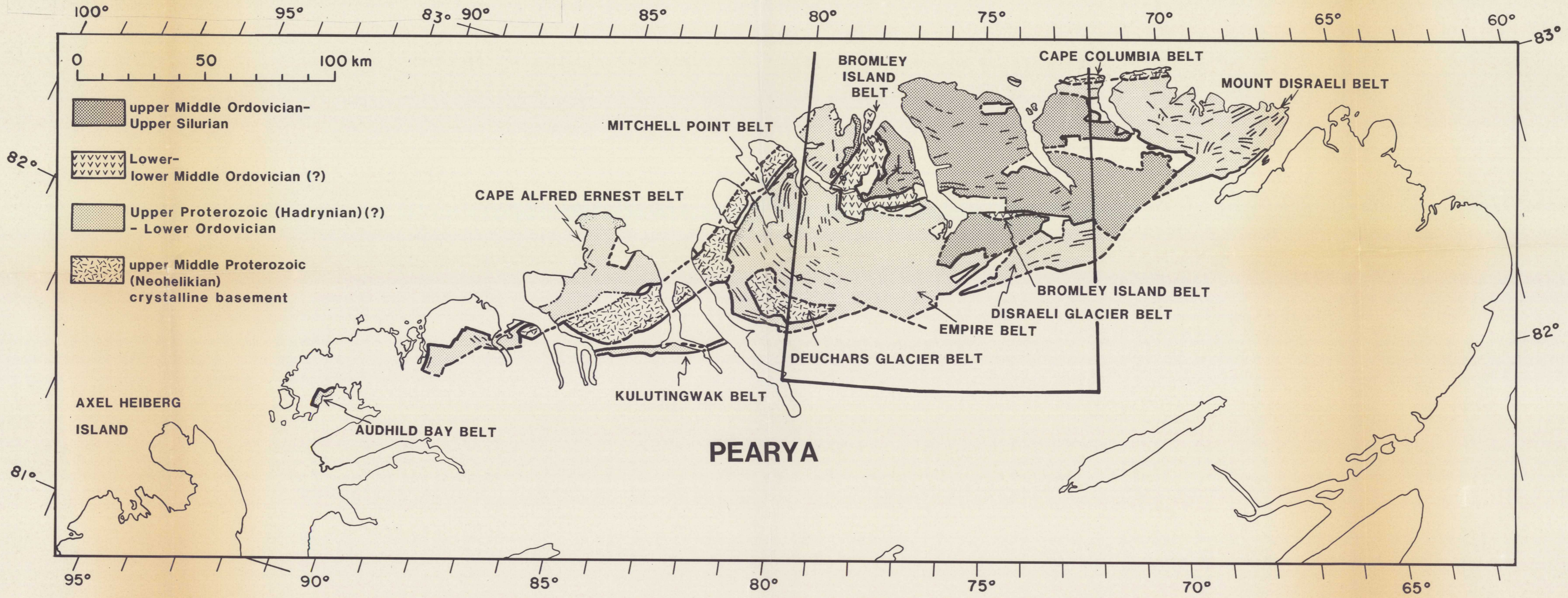
Figure 2. Subdivisions of Pearya. For structural symbols see Figure 1.
