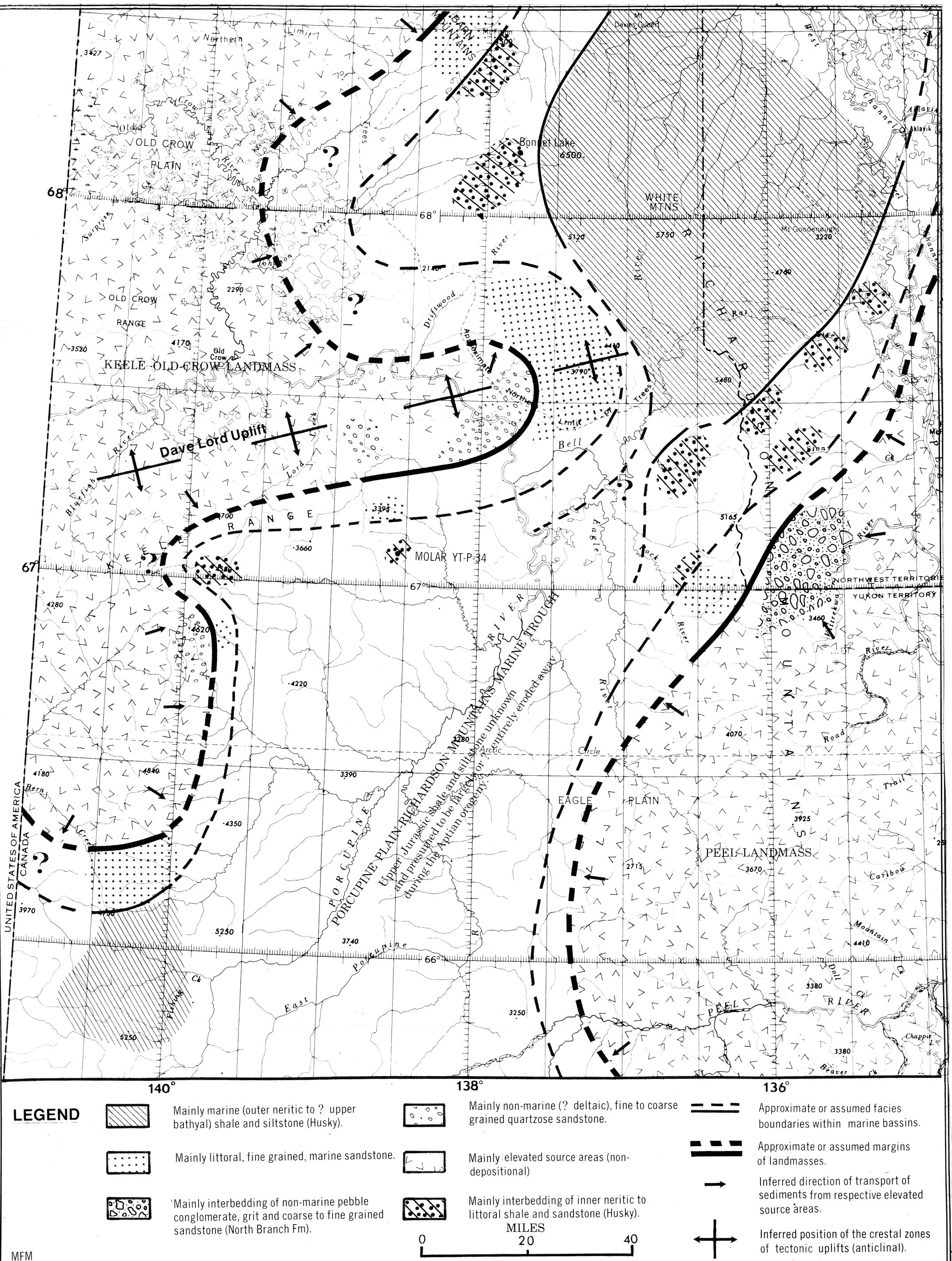
FIG. 10 Mid to Late Jurassic (Kimmeridgian to early Portlandian s.str. or time of Mid-Husky Formation and its arenaceous to rudaceous marine to non-marine equivalents) palaeogeography and depositional tectonics.
