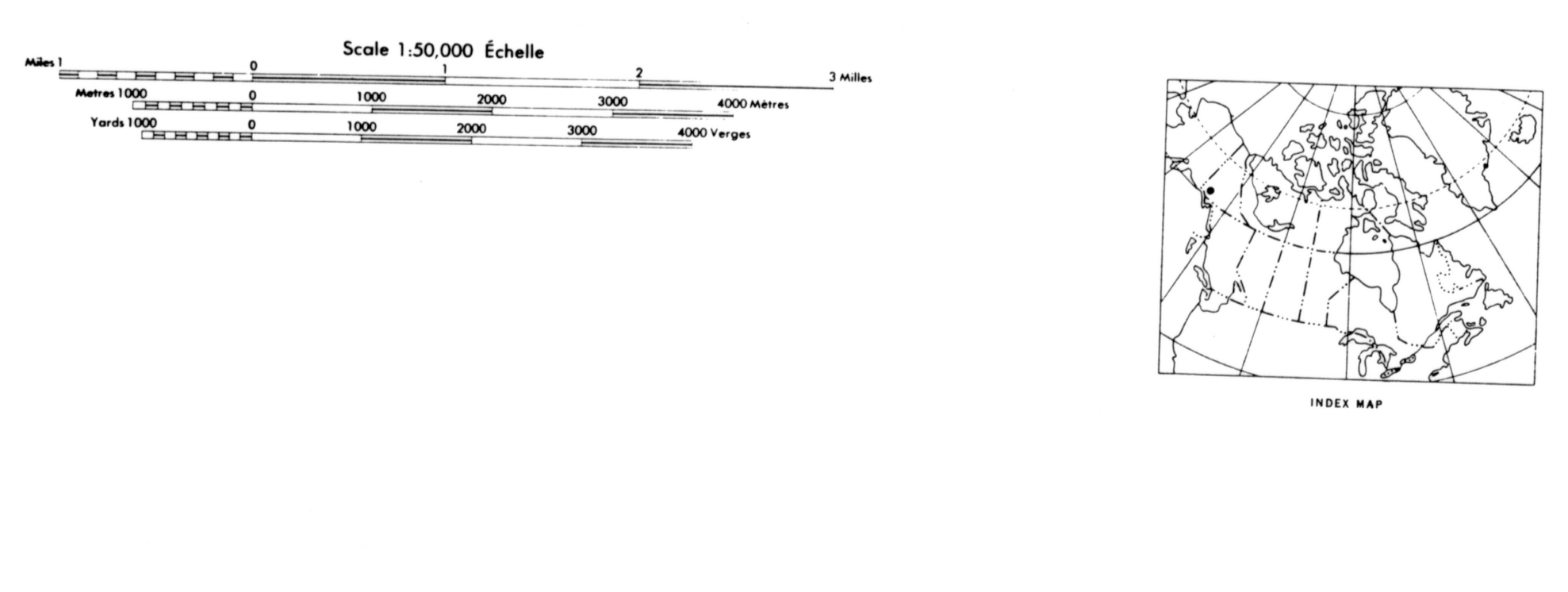
MAP 2A GEOLOGY OF PARTS OF BIGHORN CREEK (115G/3), DESTRUCTION BAY (115G/2), SLIMS RIVER (115B/15) MAP - AREAS, YUKON TERRITORY
