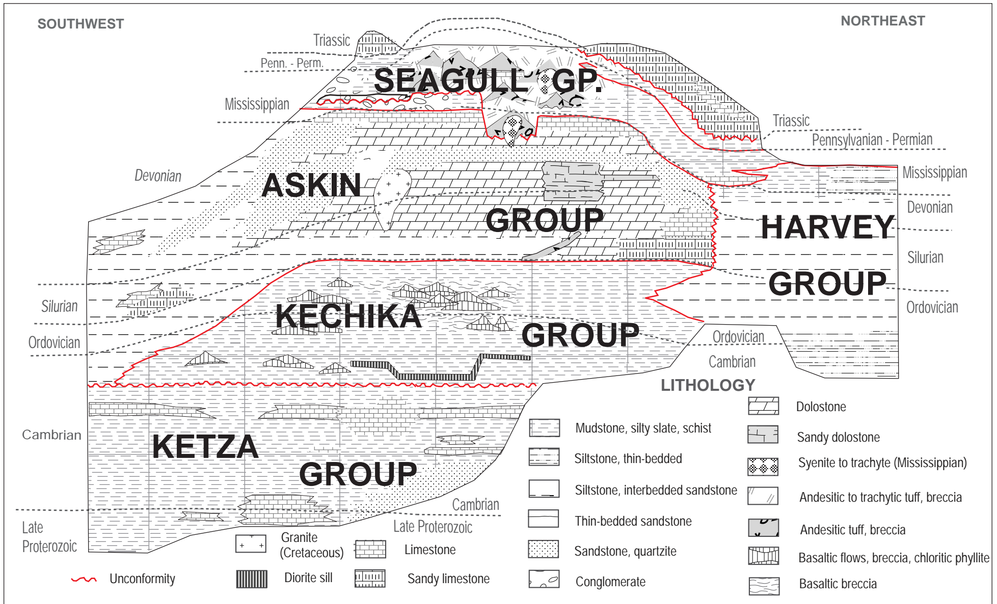
Figure 7a. Schematic diagram of principal lithologies of the Pelly-Cassiar platform, showing stratigraphic group names used in this report. [original figure re-drafted; red lines added]
