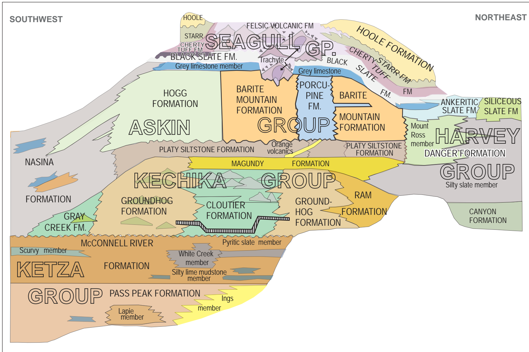
Figure 7b. Schematic diagram of formations comprising the Pelly-Cassiar platform, showing stratigraphic unit names used in this report [all formation names are informal].
