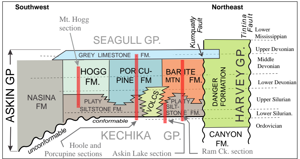
Figure 19. Schematic stratigraphic relationships of the Askin and Harvey groups. The location of stratigraphic sections (red columns) is shown on Figure 18.
