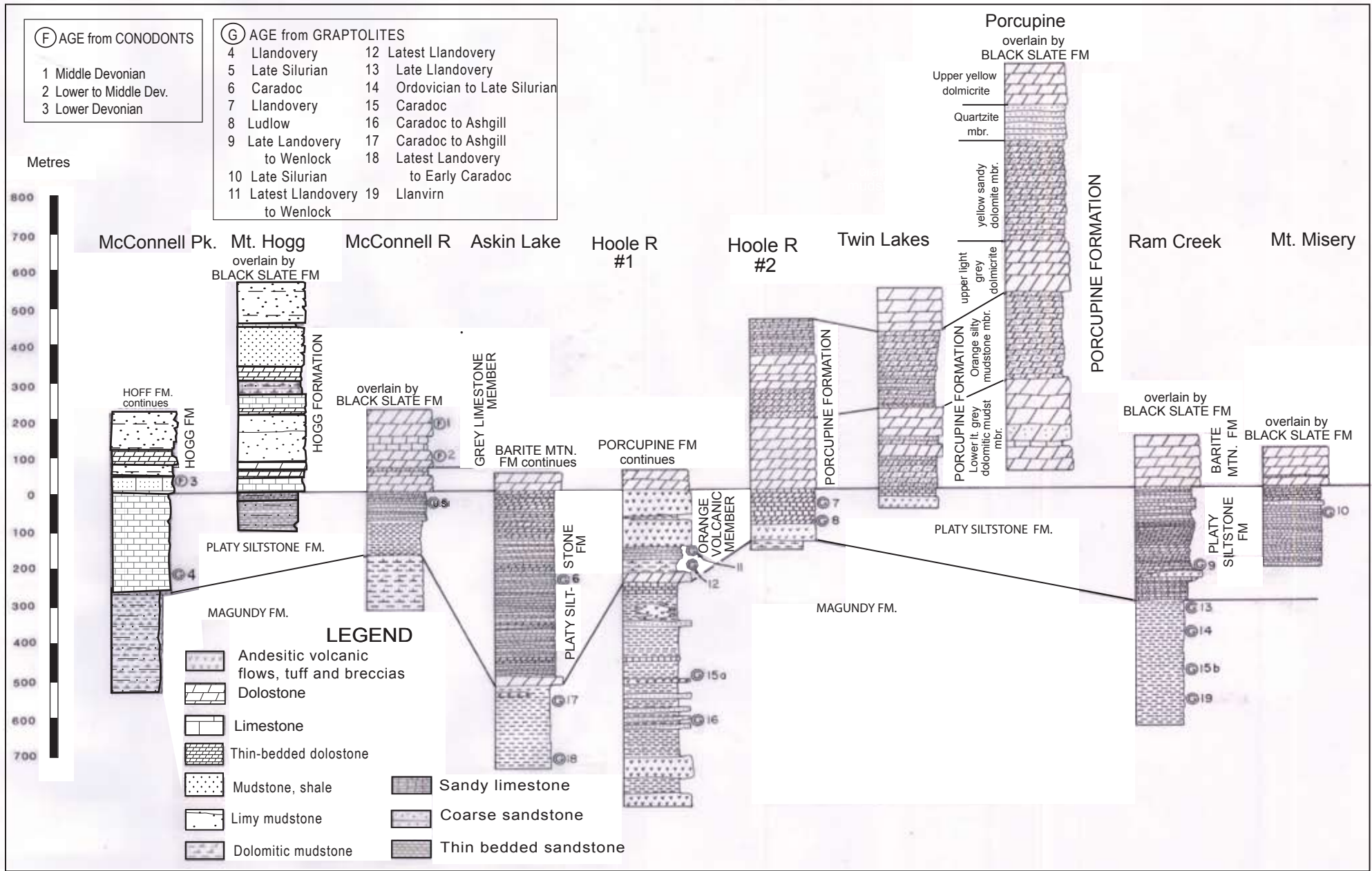
Figure 20. Fence diagram of measured stratigraphic exposures of the Askin group from different parts of the project area, showing variations in thickness and lateral discontinuity of some units. Locations of sections are shown on Figure 18.
