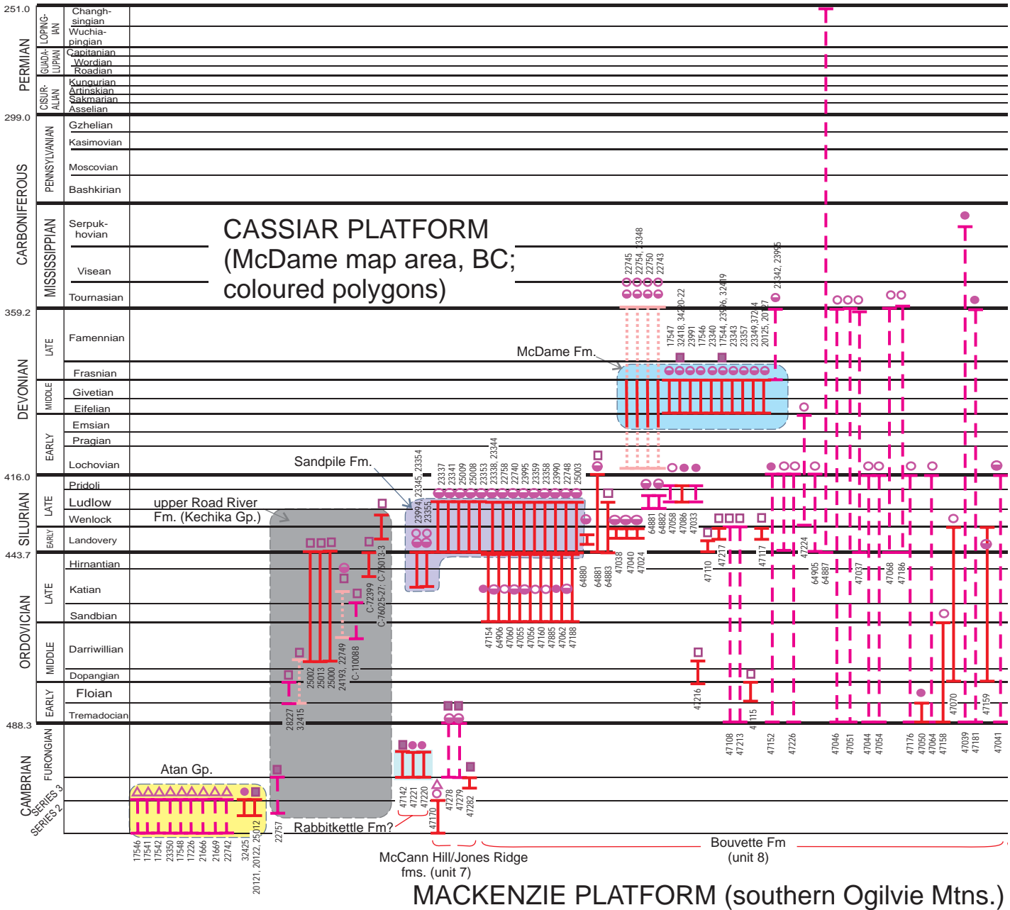
Figure 30, left half. Age range of fossil collections for selected units of the Cassiar and Mackenzie platform successions, for comparison with Quiet Lake and Finlayson Lake map areas (Fig. 12). See right half for legend. Collections cited are from Green (1972, for Mackenzie platform) and Gabrielse (1963, 1998, for Cassiar platform); documentation of collections is available from the Paleontological unit, GSC-Calgary.
