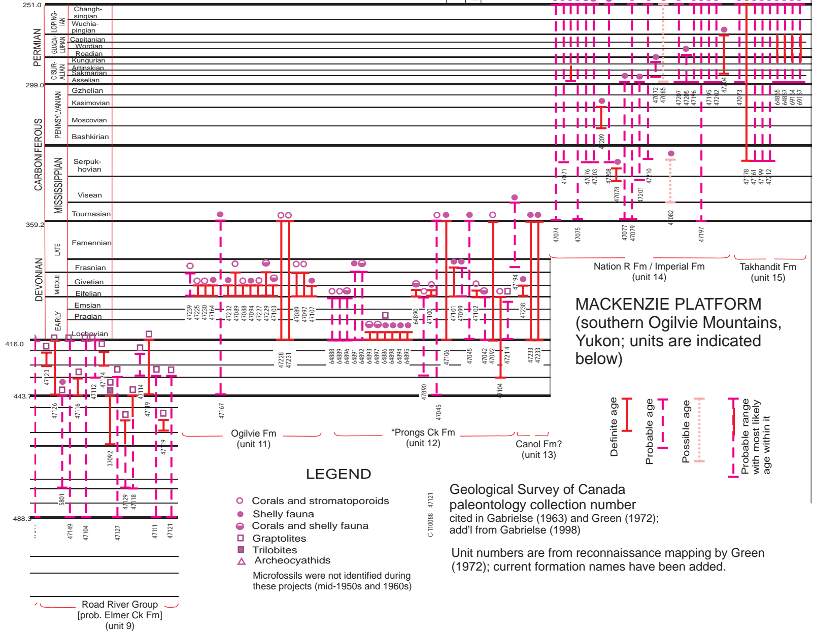
Figure 30, right half. Age range of fossil collections for selected units of the Mackenzie platform succession, for comparison with Quiet Lake and Finlayson Lake map areas (Fig. 12). Collections cited are in Green (1972); documentation of collections available from the Paleontological unit, GSC-Calgary.
