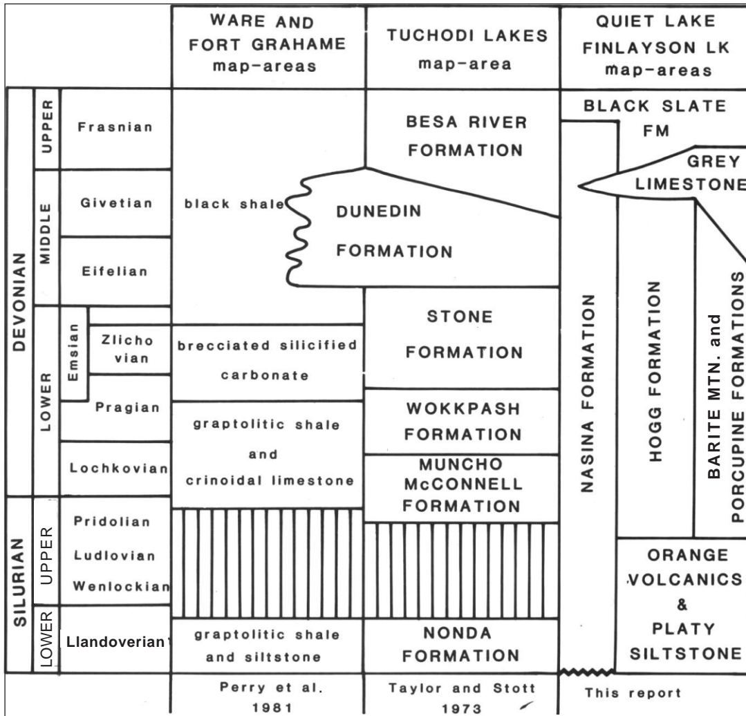
Figure 31. Correlation of the stratigraphic units of the northern Rocky Mountains with the Askin group [original figure].
