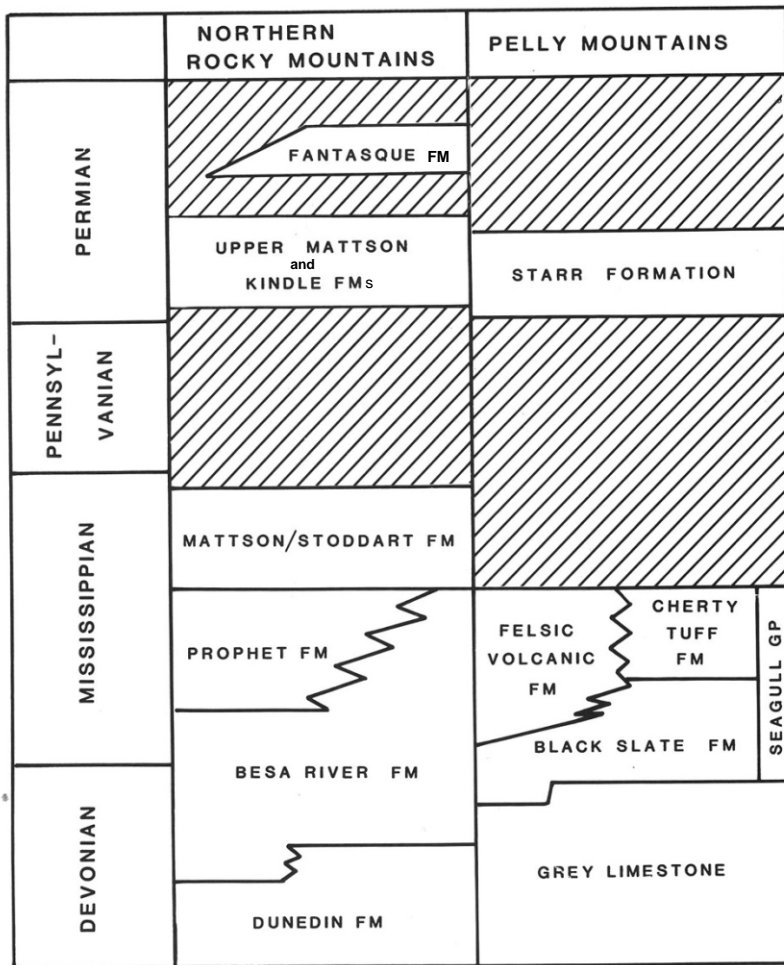
Figure 36. Correlation of the Seagull group and Starr formation with strata in the northern Rocky Mountains [original figure].
