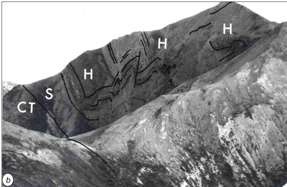
b. The Cherty Tuff (CT), Starr (S), and Hoole (H) formations are labeled in this southeast view along strike 4 km north of Mount Green. Note the recessive nature of these rocks and the disharmonic folds in the Hoole formation.
