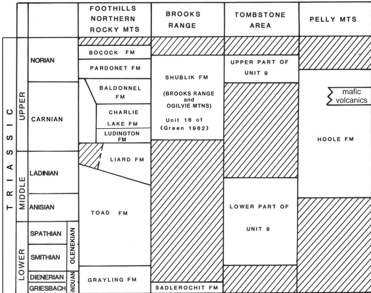
Figure 40. Correlation of the Hoole formation with time-equivalent units in the northern Canadian Cordillera [original figure].
