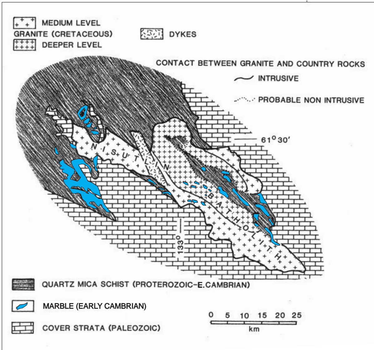
Figure 48. Regional geological setting of the Nisutlin batholith. The host schist and marble are considered equivalent to the Ketzá group. Part of the batholith intrudes the surrounding metamorphic rocks, but other parts appear gradational with host rocks. The carbonate can be traced from the east side of the intrusion to the metamorphic rocks on the west. [coloured original figure]
