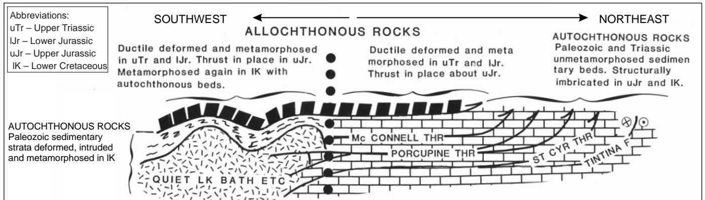
Figure 51. Schematic structural transect of the project area southwest of Tintina fault. The same allochthonous rocks rest above autochthonous strata, but different features are present in the northeast and southwest regions. In the northeast the allochthonous slice rests on an imbricated, but unmetamorphosed, stratigraphic stack. To the southwest the allochthonous rocks structurally overlie metamorphosed and intruded autochthonous strata, and are deformed with them [original figure].
