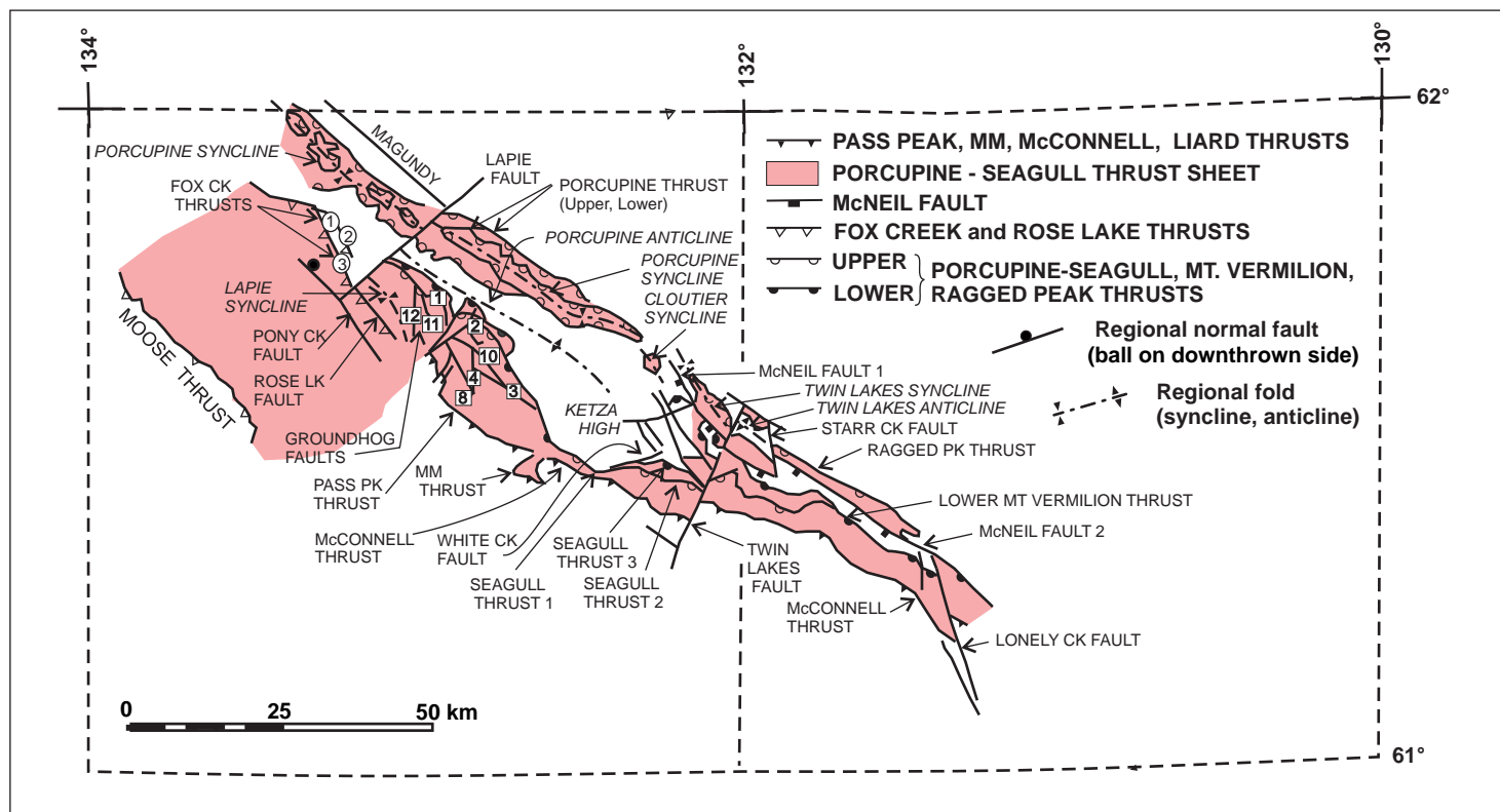
Figure 53. Map of the Porcupine-Seagull thrust sheet and its main structures. The sheet is bounded above by the McConnell and related thrusts, and below by the Porcupine-Seagull thrusts. These sole thrusts may merge in the western part of area. Groundhog faults (numbers in squares) are simplified here [the complete set are shown on sheet 7 (105F/15; Ram Creek; 1:50 000 scale)].
