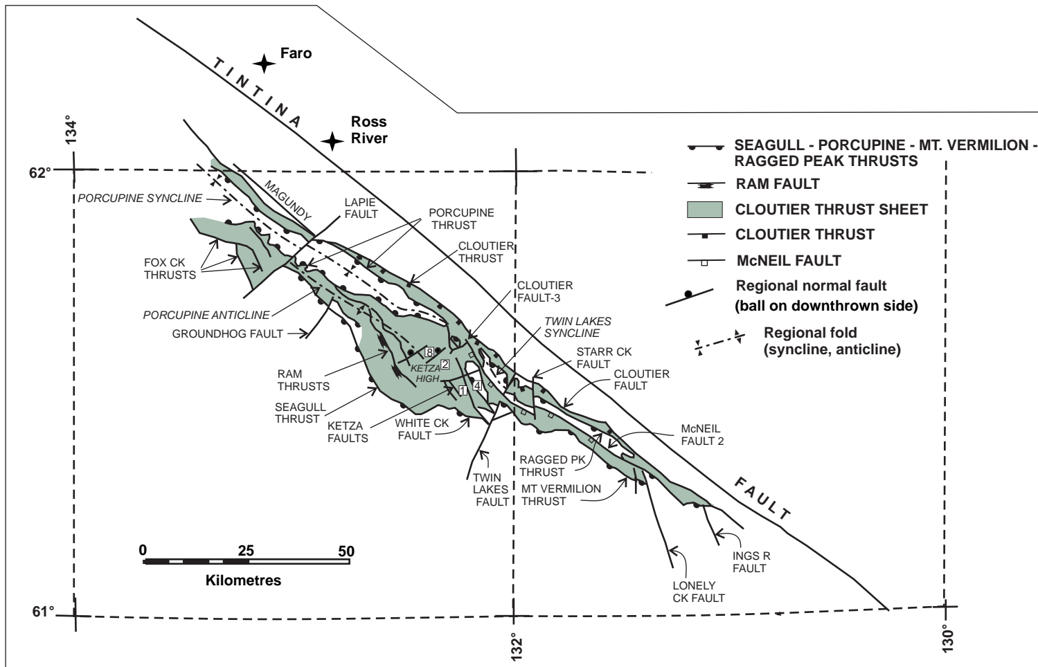
Figure 62. Map of Cloutier thrust sheet and its main structures. The sheet lies between the Cloutier and Seagull-Porcupine-Mt. Vermilion-Ragged Peak thrusts. It is cut by splays of lower thrusts, and folded by structures that probably die downward on the St. Cyr thrust. Some of the Ketzka faults (numbered) are shown here [the complete set of faults are shown on sheet 4 (105F/9 – Cloutier Creek; 1:50 000 scale)].
