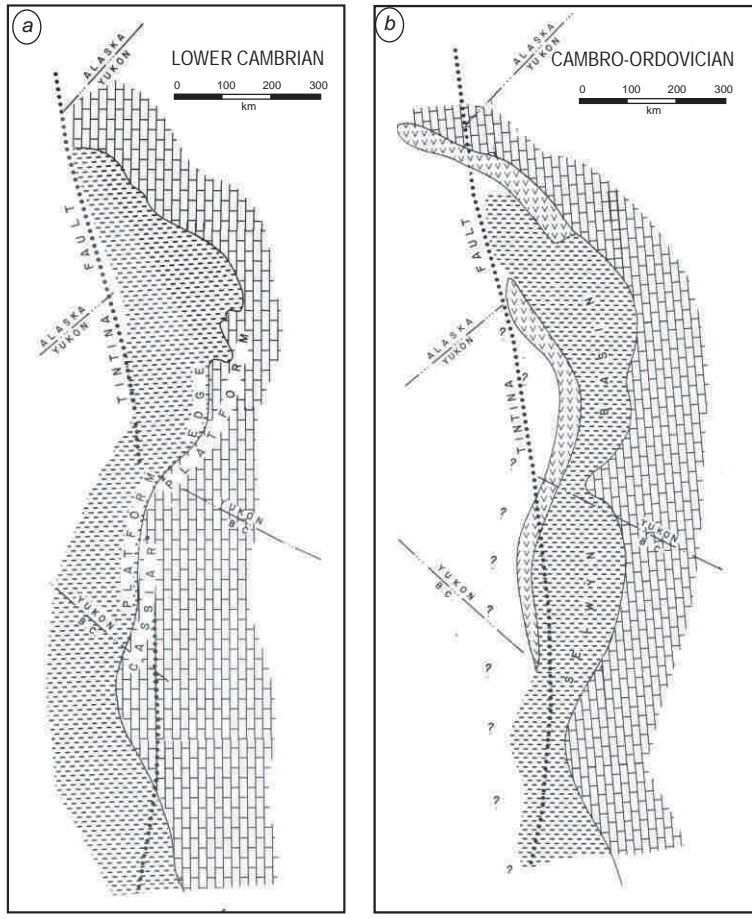
Figure 68. Schematic facies distribution of the autochthonous strata at different time periods, with 450 km dextral slip on the Tintina fault restored. Each stratigraphic assemblage was displaced by roughly the same distance along Tintina fault, implying that fault movement postdated deposition.
