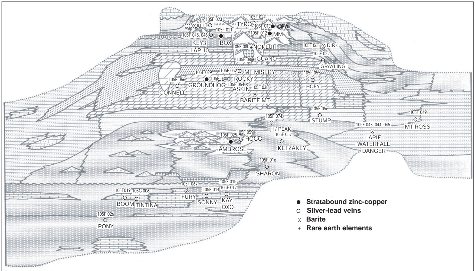
Figure 70. The lithologic association and stratigraphic position of selected mineral showings in the Pelly-Cassiar platform. Symbols represent different occurrence types, their numbers correspond to Yukon Minfile, and lithology patterns from Figure 7a.
