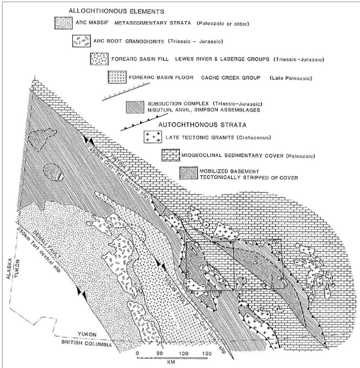
Figure 74. Schematic map of southern Yukon showing the distribution of rock units that are interpreted as elements of the Lewes River arc. The relationship of autochthonous basement and supracrustal rocks to obducted arc elements is depicted. The project area is outlined [original figure].
