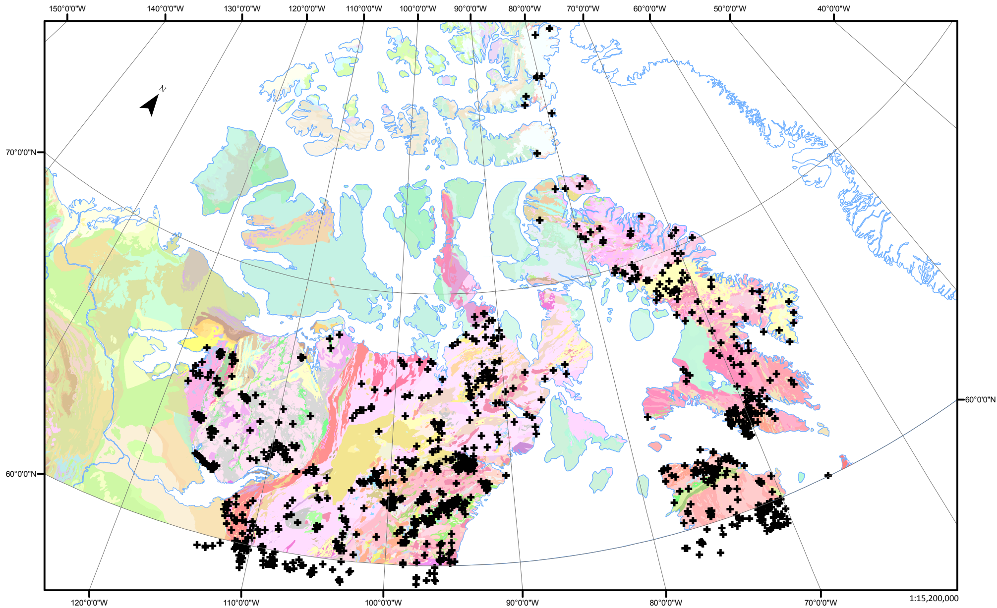
Figure 1. Map of northern Canada showing distribution of all Sm-Nd isotopic data. The data points are superimposed onto the Canadian onshore segment of the Geologic Map of the Arctic by Harrison et al. (in press).
