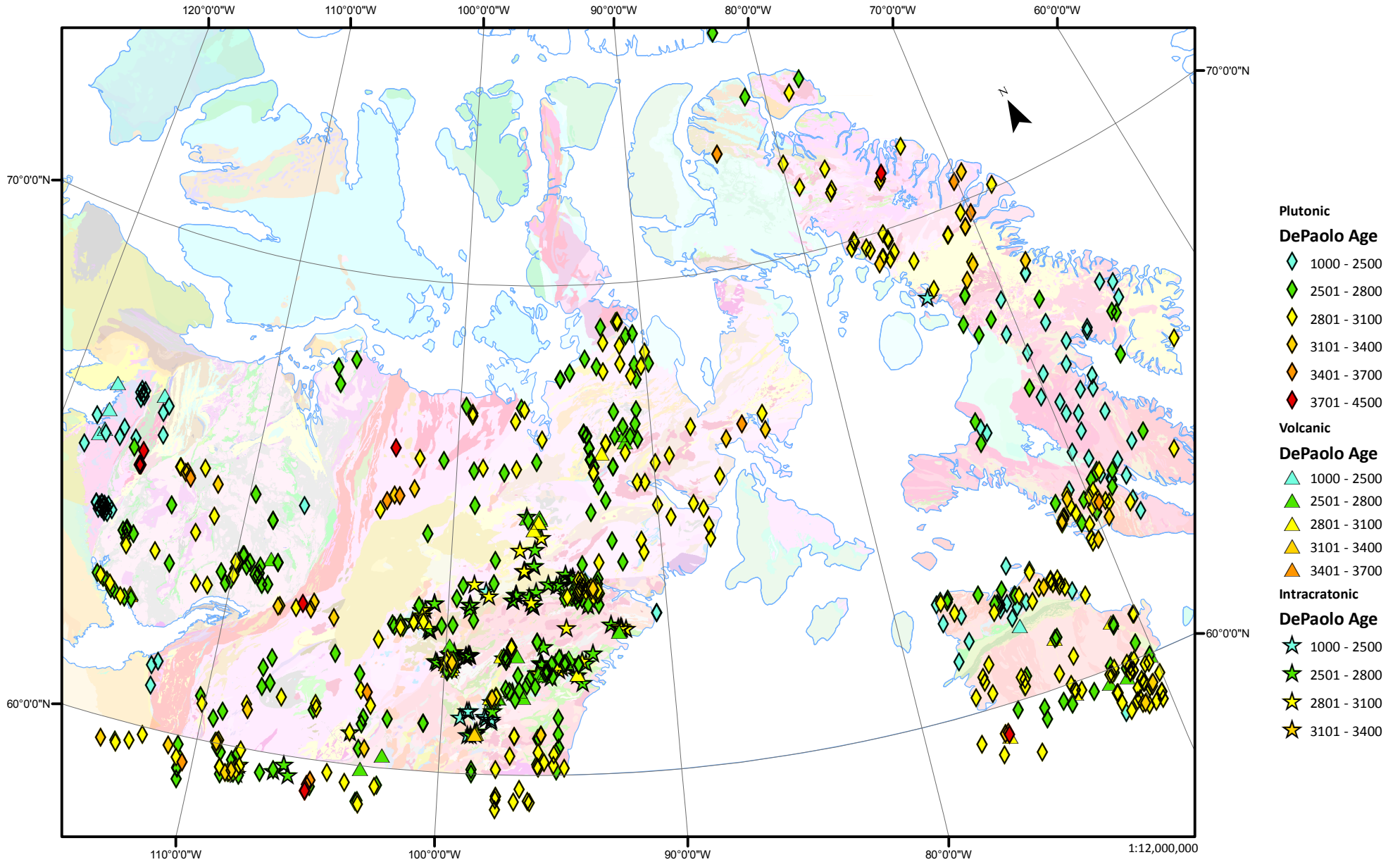
Figure 2. Depleted mantle model ages (DePaolo, 1981) for Sm-Nd isotopic data analyses of two rock types (Plutonic, Volcanic) and one rock association (Intracratonic); each group is further categorized into a total of six DePaolo Age intervals ranging from the Proterozoic to the Hadean. The data points are superimposed onto the Canadian onshore segment of the Geologic Map of the Arctic by Harrison et al. (in press).
