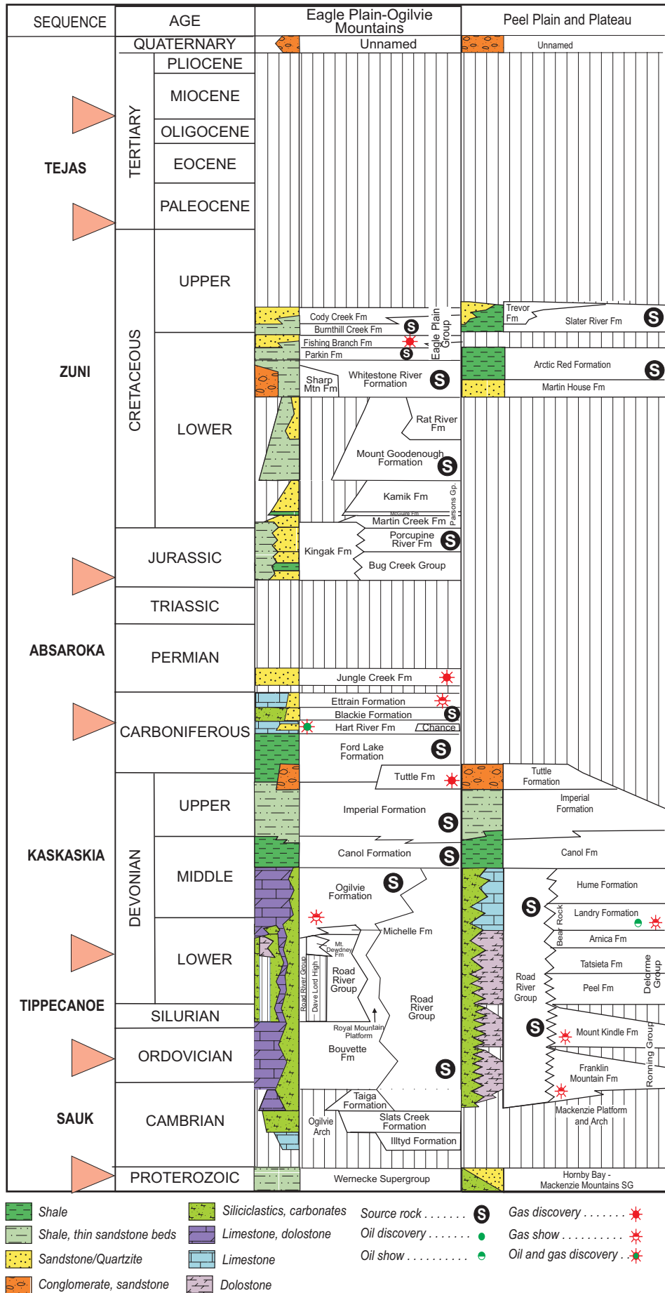
Figure 2. Correlation chart of sedimentary strata in Eagle Plain basin and Peel Plateau and Plain. Petroleum discoveries, shows and known and potential source rocks are indicated. From Morrow (1999), Dixon (1999), Pugh (1993), Hadlari et al. (2009a, 2009b) and Haggart et al. (2013).
