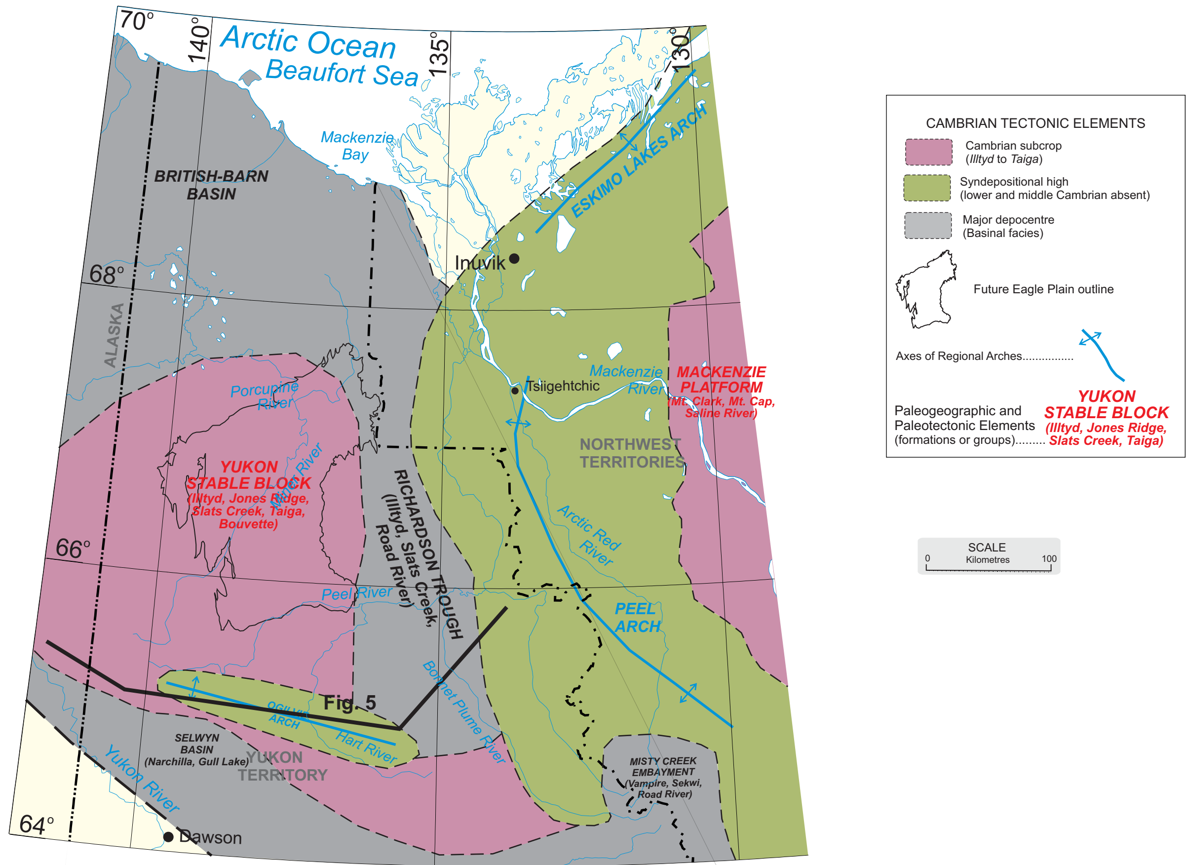
Figure 3. Paleogeographic map of Cambrian strata (Illyd to Taiga interval) with major tectonic elements. From Fritz et al. (1991); Lane (1991); Aitken (1993); Cecile et al. (1997); Morrow (1999). Section line of Figure 5 is depicted.
