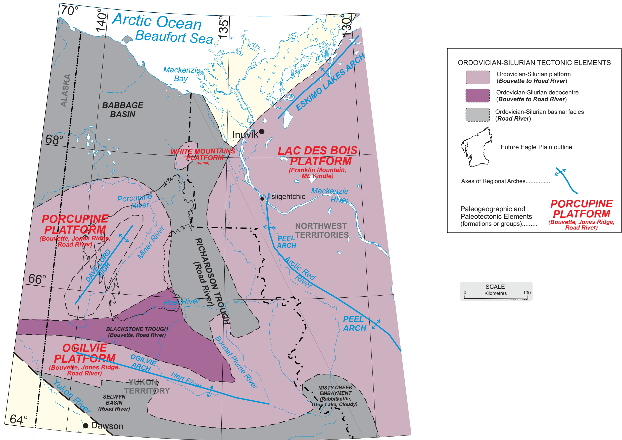
Figure 4. Paleogeographic-facies map of Ordovician and Silurian strata (Bouvette to Road River interval) with major tectonic elements. From Wheeler and McFeeley (1991); Lane (1991); Cecile et al. (1997); Norford (1997); Morrow (1989; 1999).
