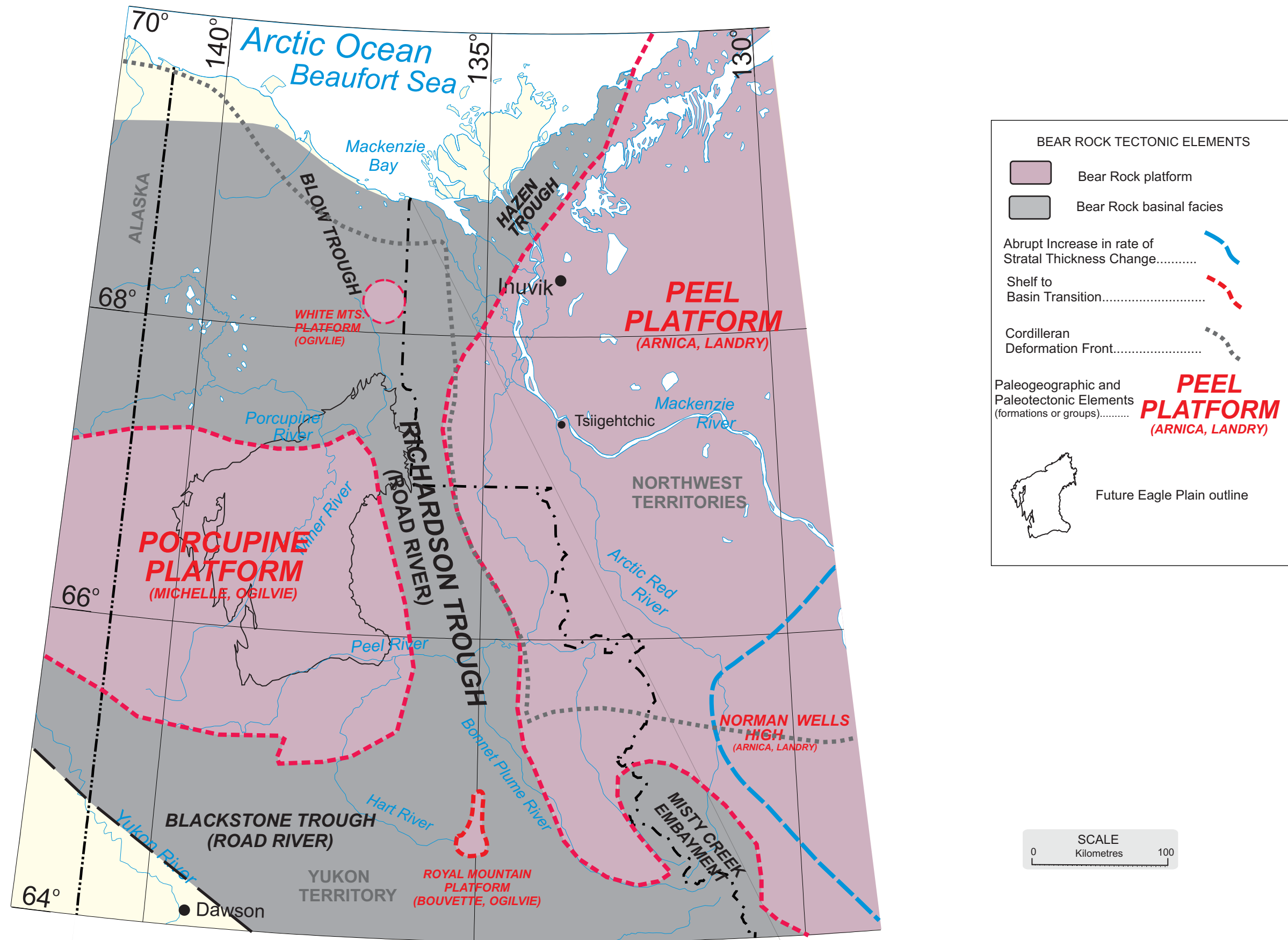
Figure 7. Paleogeographic-facies map of Early to Middle Devonian Bear Rock assemblage with major tectonic elements. From Fritz et al., (1991); Norris (1997); Morrow (1999).
