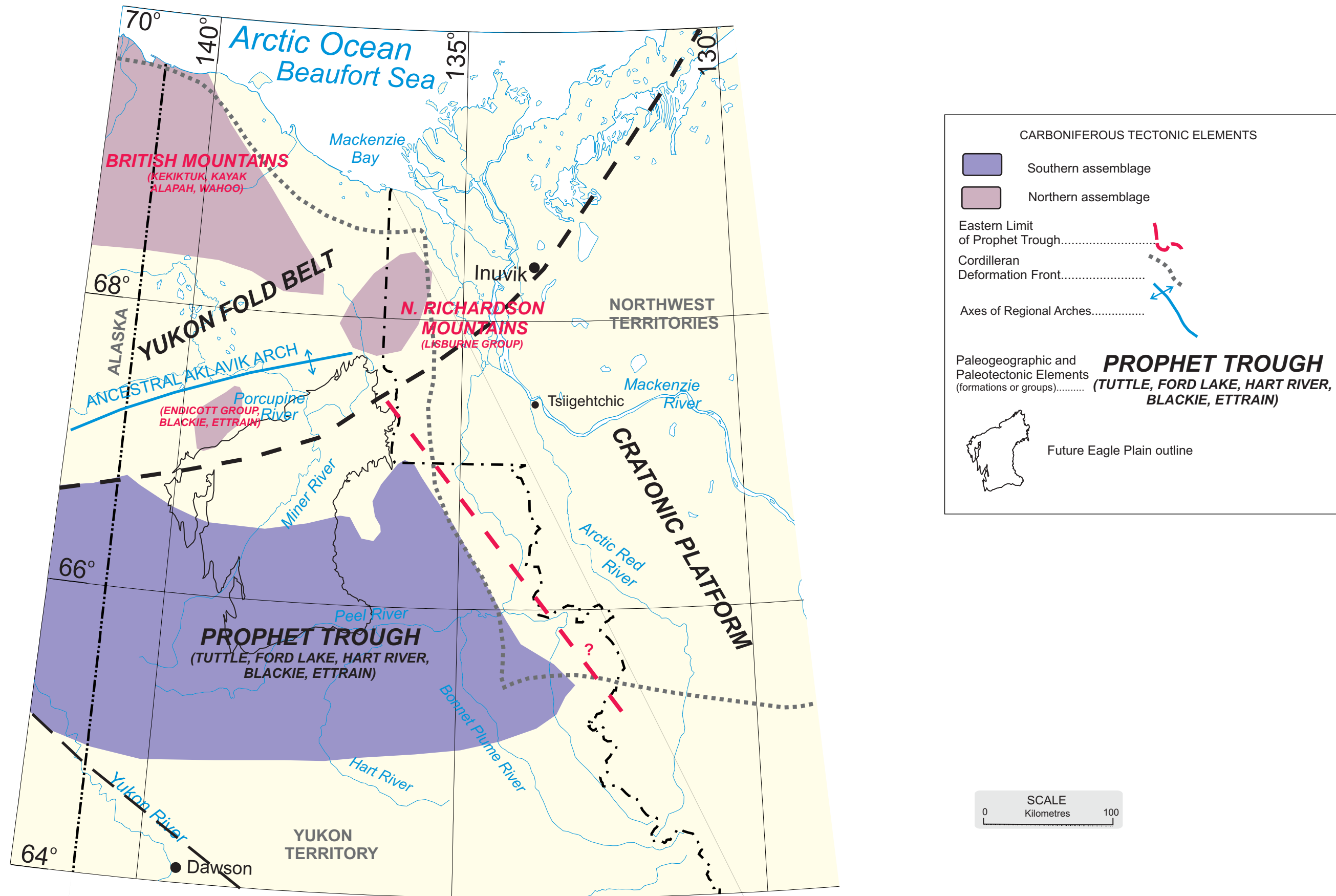
Figure 11. Assemblage map of Carboniferous sedimentary units with major tectonic elements. From Gordey et al., (1991); Richards et al., (1997).
