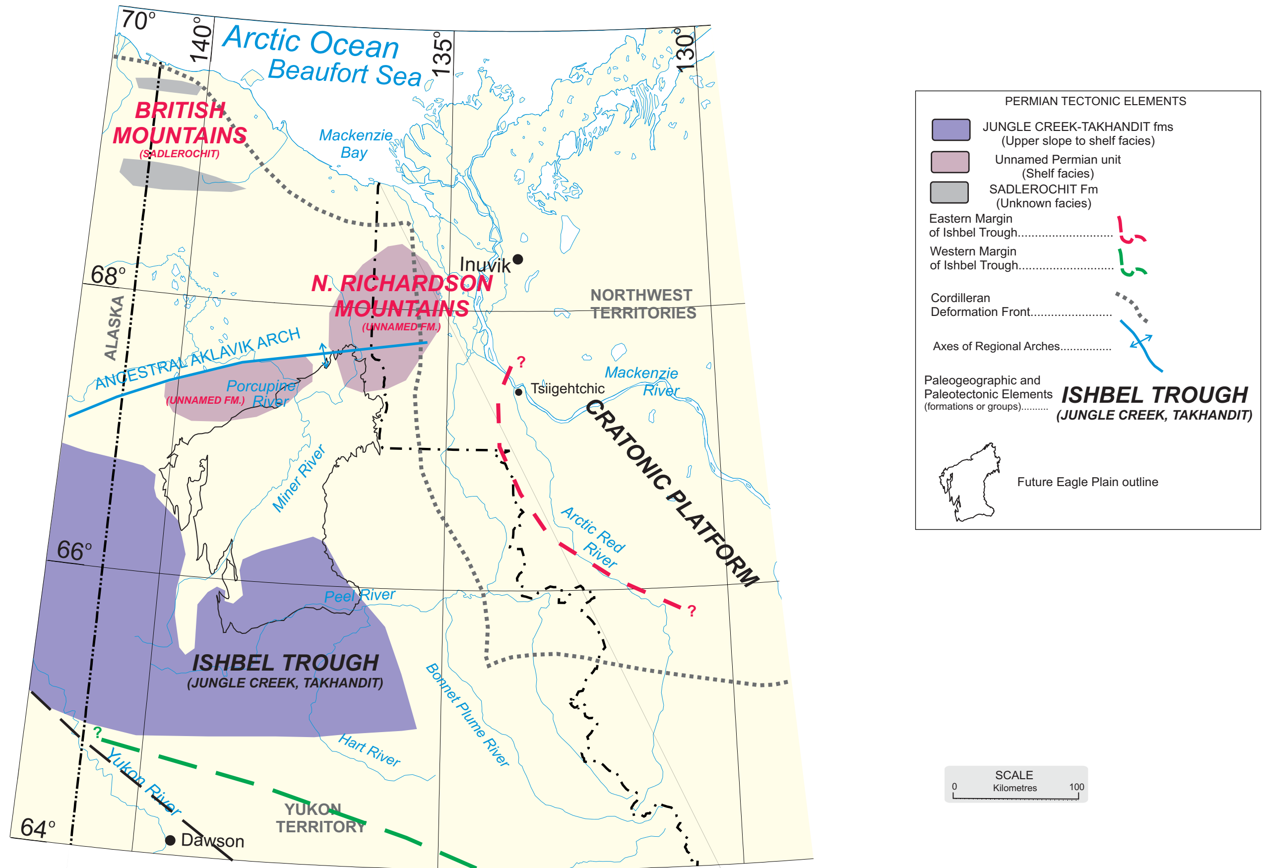
Figure 12. Facies distribution map of Permian units with major tectonic elements. From Gordey et al., (1991); Richards et al., (1997).
