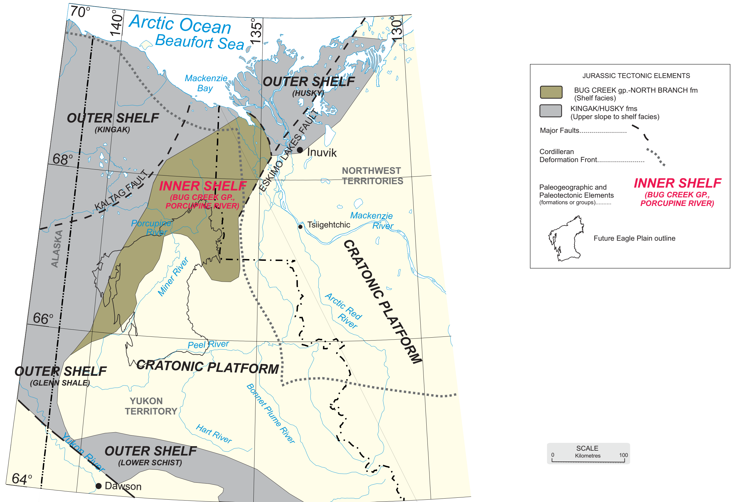
Figure 13. Facies distribution map of Jurassic units with major tectonic elements. From Gordey et al., (1991); Poulton (1997).
