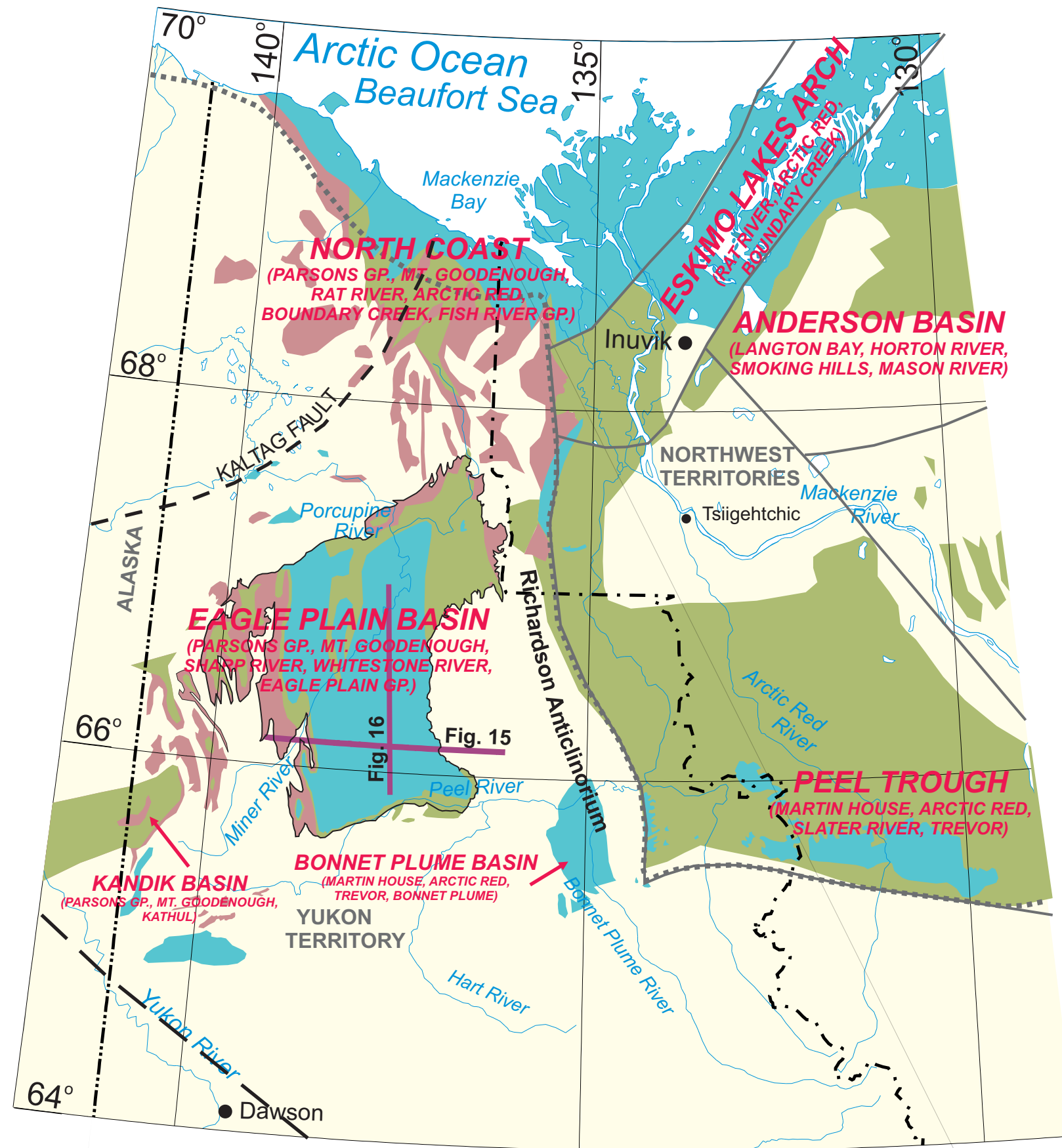
Figure 14. Geologic bedrock and subcrop map of Cretaceous-Paleogene units with major tectonic elements. From Yorath (1991); Dixon (1992; 1997). Lines of schematic cross-sections are shown.
