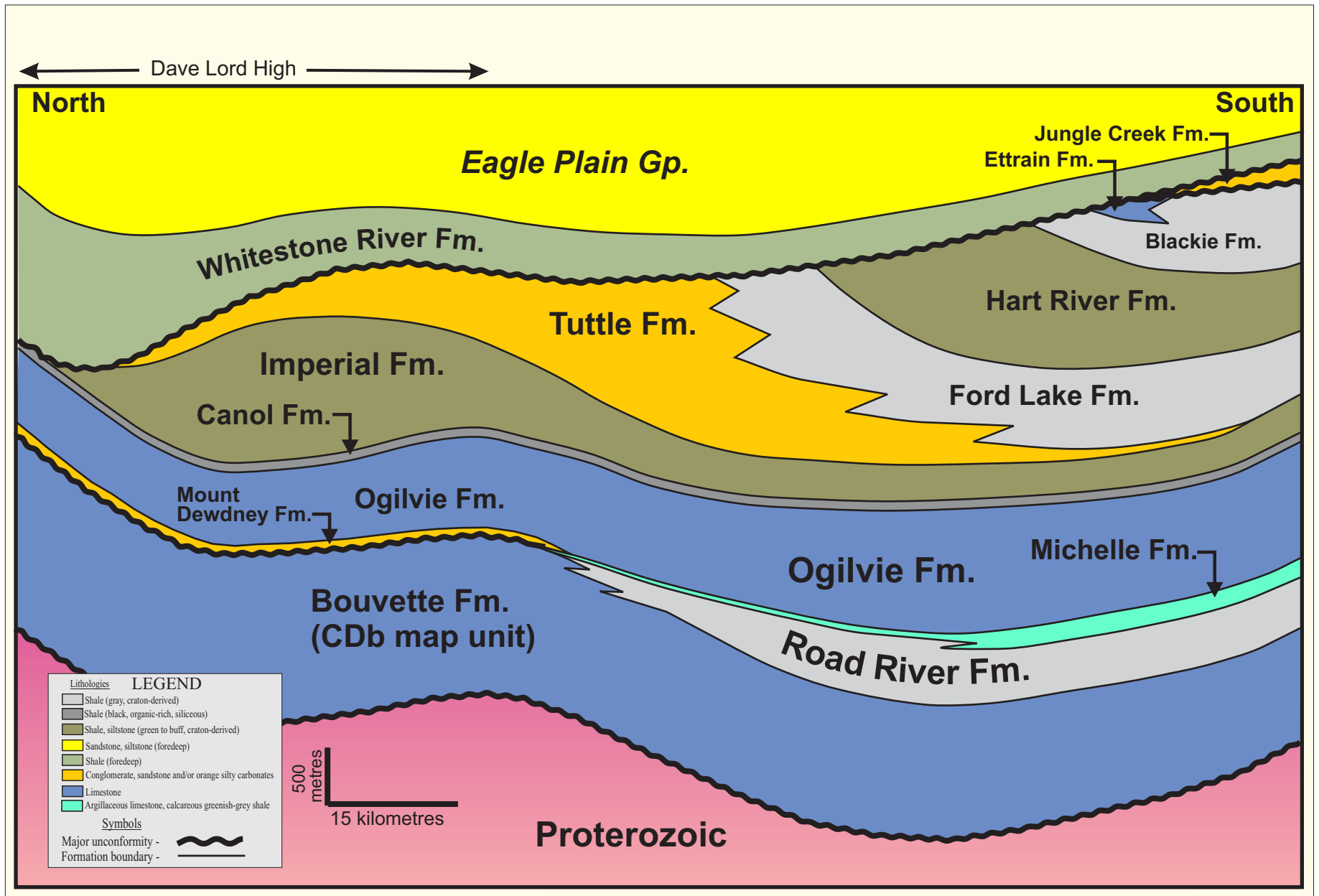
Figure 16. A north-south schematic cross-section across Eagle Plain basin and the south flank of Eagle Arch. Section line depicted on Fig. 14.
