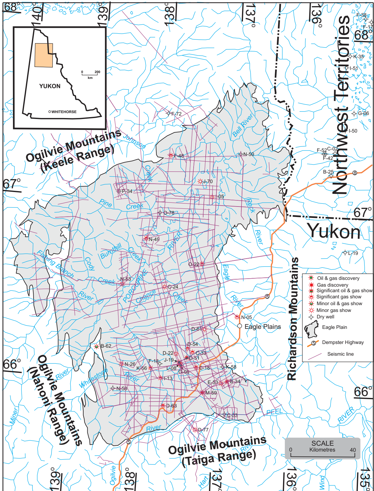
Figure 18. Petroleum wells completed in the Eagle Plain basin. Major discovery locations are illustrated. Publicly available reflection seismic lines of all vintages are also depicted.
