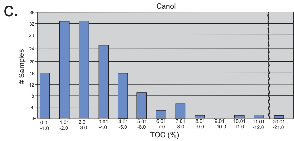
Figure 19. Histograms of frequency distribution of total organic carbon (TOC) and HI vs OI (pseudo-van Krevelen) plots for selected Lower Paleozoic source rocks (a. Road River Gp., b. Ogilvie, and c. Canol fms.).
