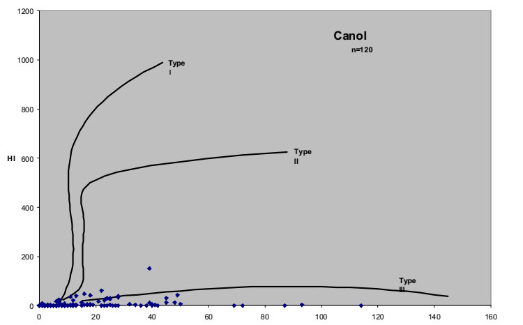
Figure 19. Histograms of frequency distribution of total organic carbon (TOC) and HI vs OI (pseudo-van Krevelen) plots for selected Lower Paleozoic source rocks (a. Road River Gp., b. Ogilvie, and c. Canol fms.).
