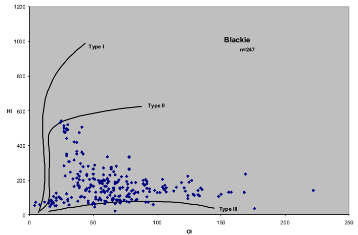
Figure 20. Histograms of frequency distribution of total organic carbon (TOC) and HI vs OI (pseudo-van Krevelen) plots for selected Upper Paleozoic source rocks (a. Imperial, b. Ford Lake, c. Hart River, and d. Blackie fms.).
