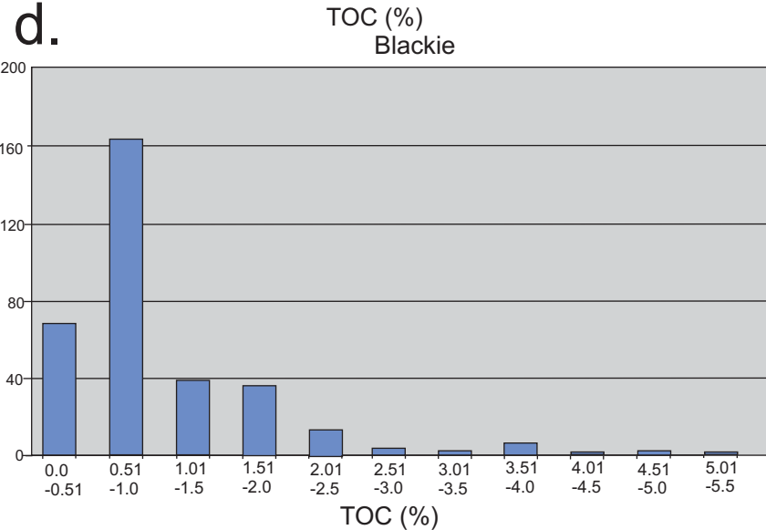
Figure 20. Histograms of frequency distribution of total organic carbon (TOC) and HI vs OI (pseudo-van Krevelen) plots for selected Upper Paleozoic source rocks (a. Imperial, b. Ford Lake, c. Hart River, and d. Blackie fms.).
