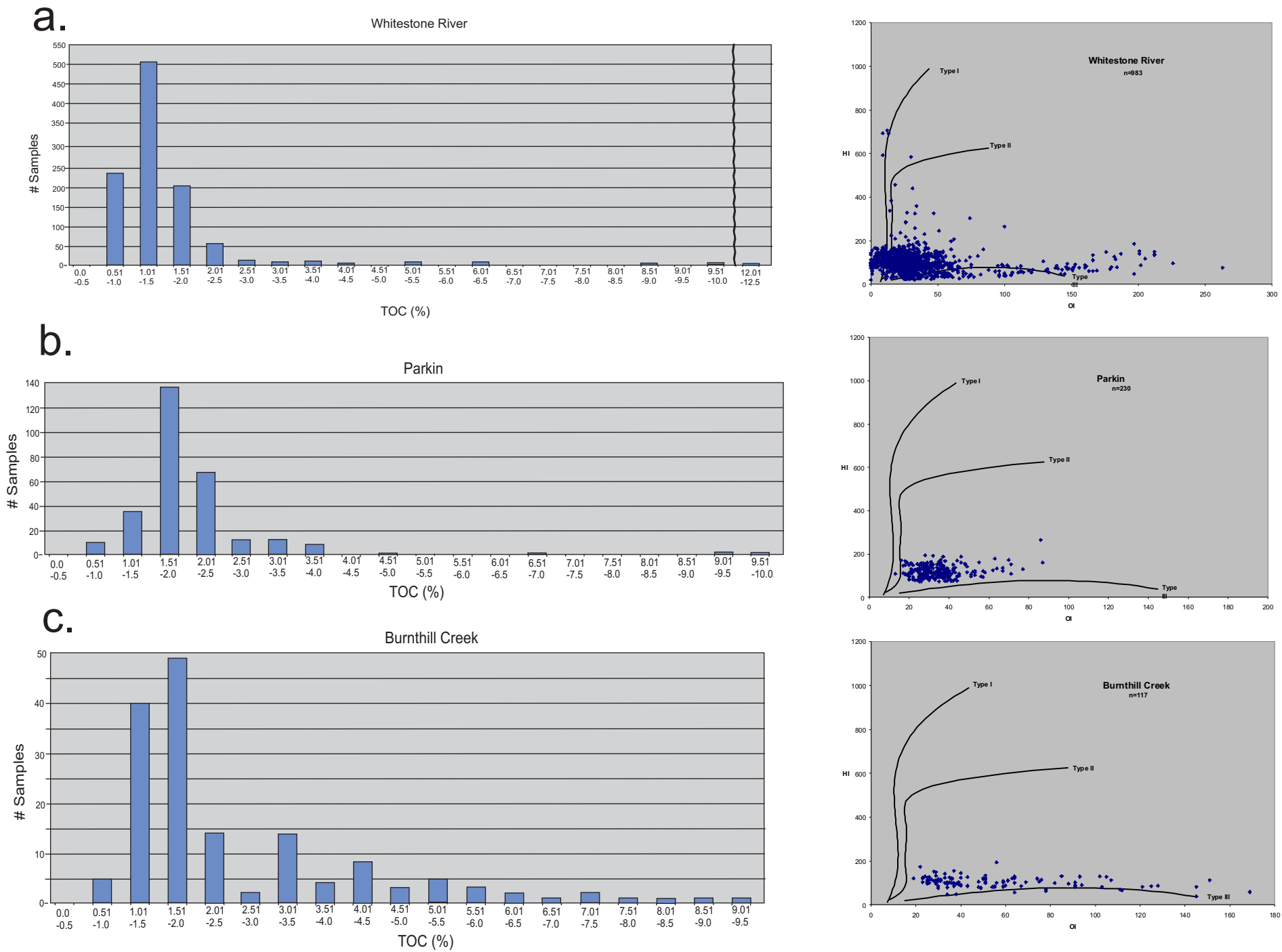
Figure 21. Histograms of frequency distribution of total organic carbon (TOC) and HI vs OI (pseudo-van Krevelen) plots for selected Cretaceous source rocks (a. Whitestone River, b. Parkin, and c. Burnthill Creek fms.).
