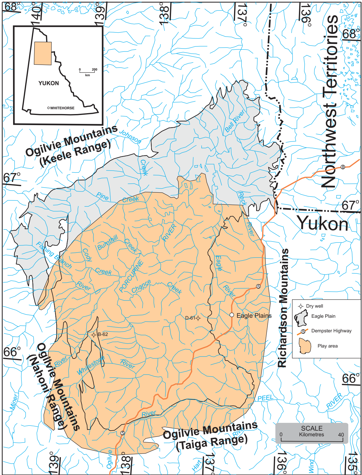
Figure 22. Lower Paleozoic carbonate pre-Laramide structural gas play.
