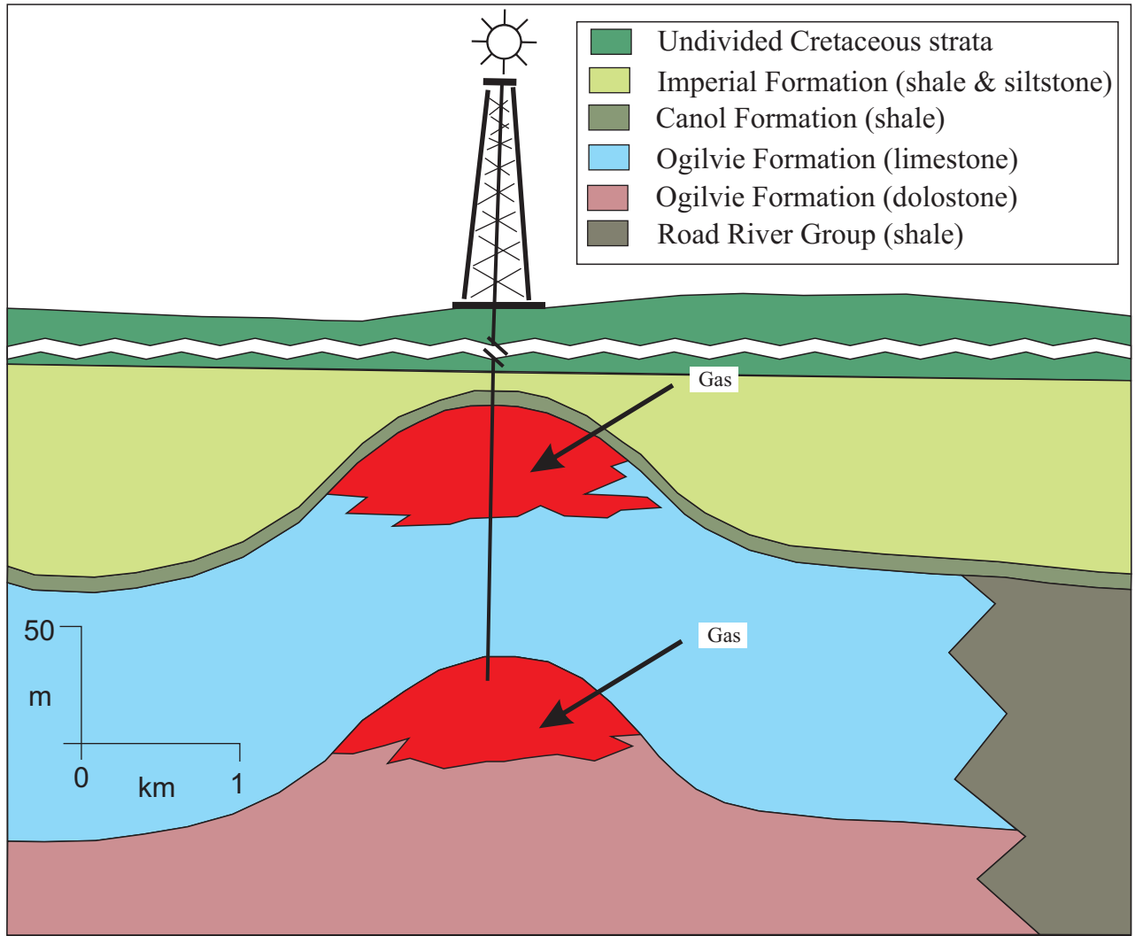
Figure 23. Schematic cross-section illustrating potential trap configurations in the Lower Paleozoic pre-Laramide structural gas play. Illustrated traps include anticlinal traps. From National Energy Board, 2000.
