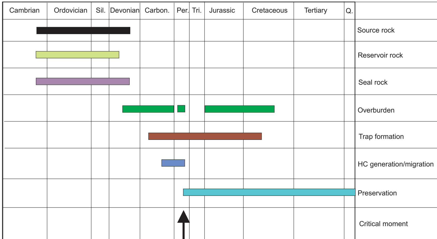
Figure 24. Petroleum event chart for a Lower Paleozoic petroleum system (Road River/Ogilvie/Canol source-Bouvette/Ogilvie reservoir). The critical moment for oil and gas generation (arrow) occurred during Early Permian time as a result of uplift of the Richardson Mountains anticlinorium and associated tectonic development of contractional fold and fault structures in Eagle Plains to the west (Link and Bustin, 1989; Hall and Cook, 1998). Sil.-Silurian, Carbon.-Carboniferous, Per.-Permian, Tri.-Triassic, Q.-Quaternary.
