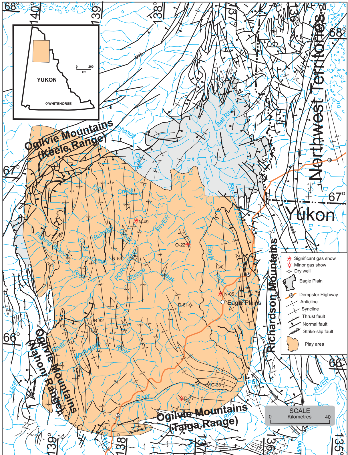
Figure 26. Lower Paleozoic carbonate Laramide structural gas play. Laramide surface structures are depicted.
