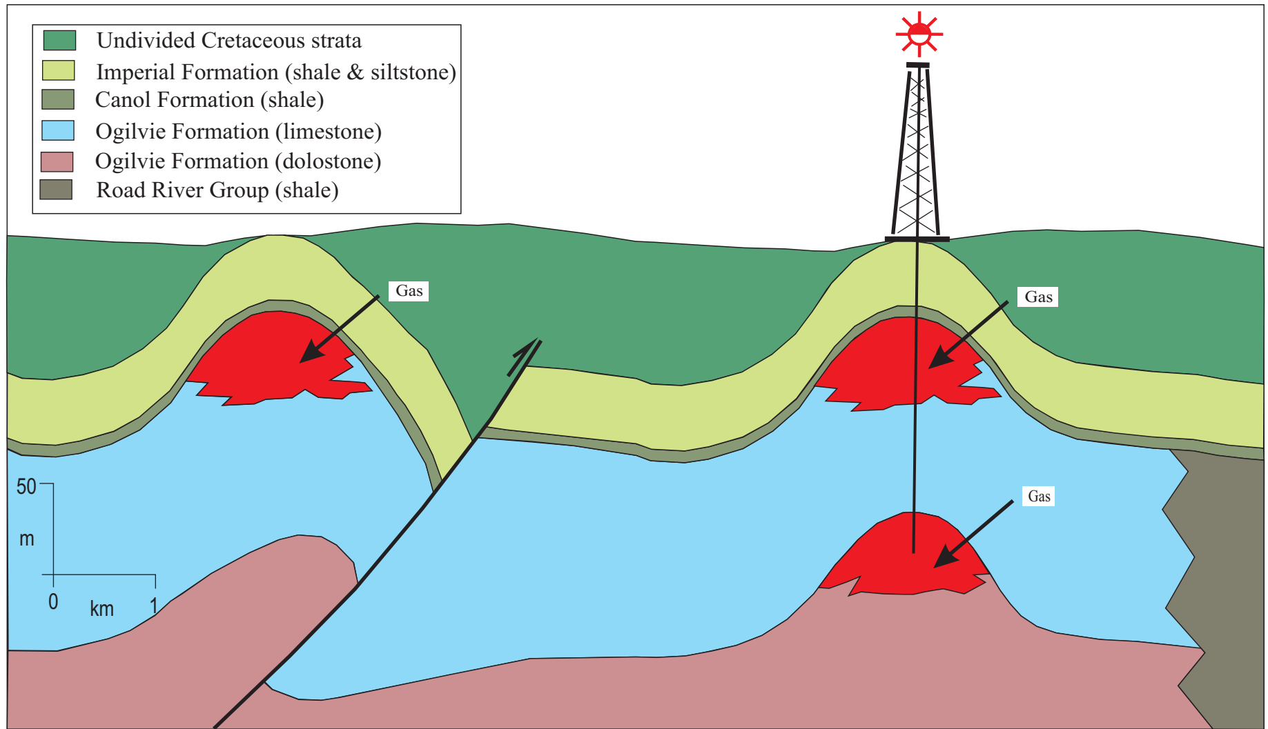
Figure 27. Schematic cross-section illustrating potential trap configurations in the Lower Paleozoic Laramide structural gas play. Illustrated traps include antiformal structures..
