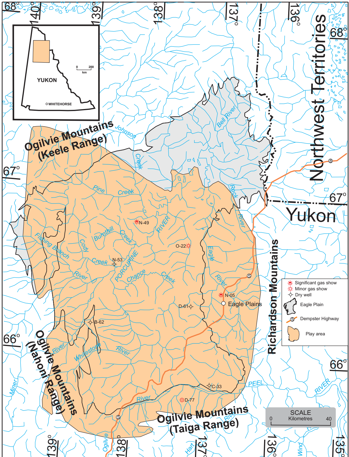
Figure 30. Lower Paleozoic carbonate stratigraphic gas play.
