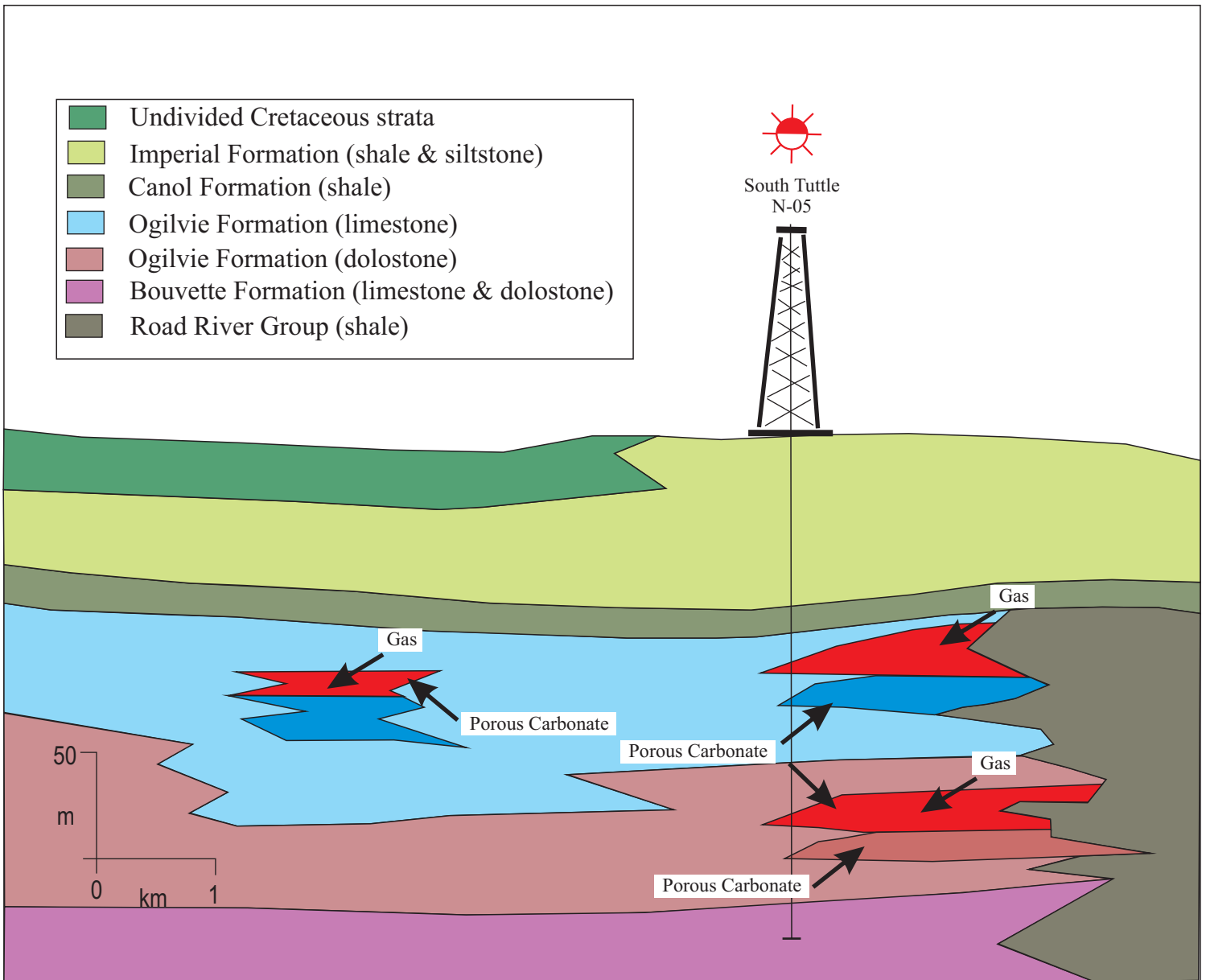
Figure 31. Schematic cross-section illustrating potential trap configurations in the Lower Paleozoic stratigraphic gas play. Illustrated traps include facies change traps where porous carbonates abut against tight basinal shale or non-porous carbonate within the formation. From National Energy Board, 2000.
