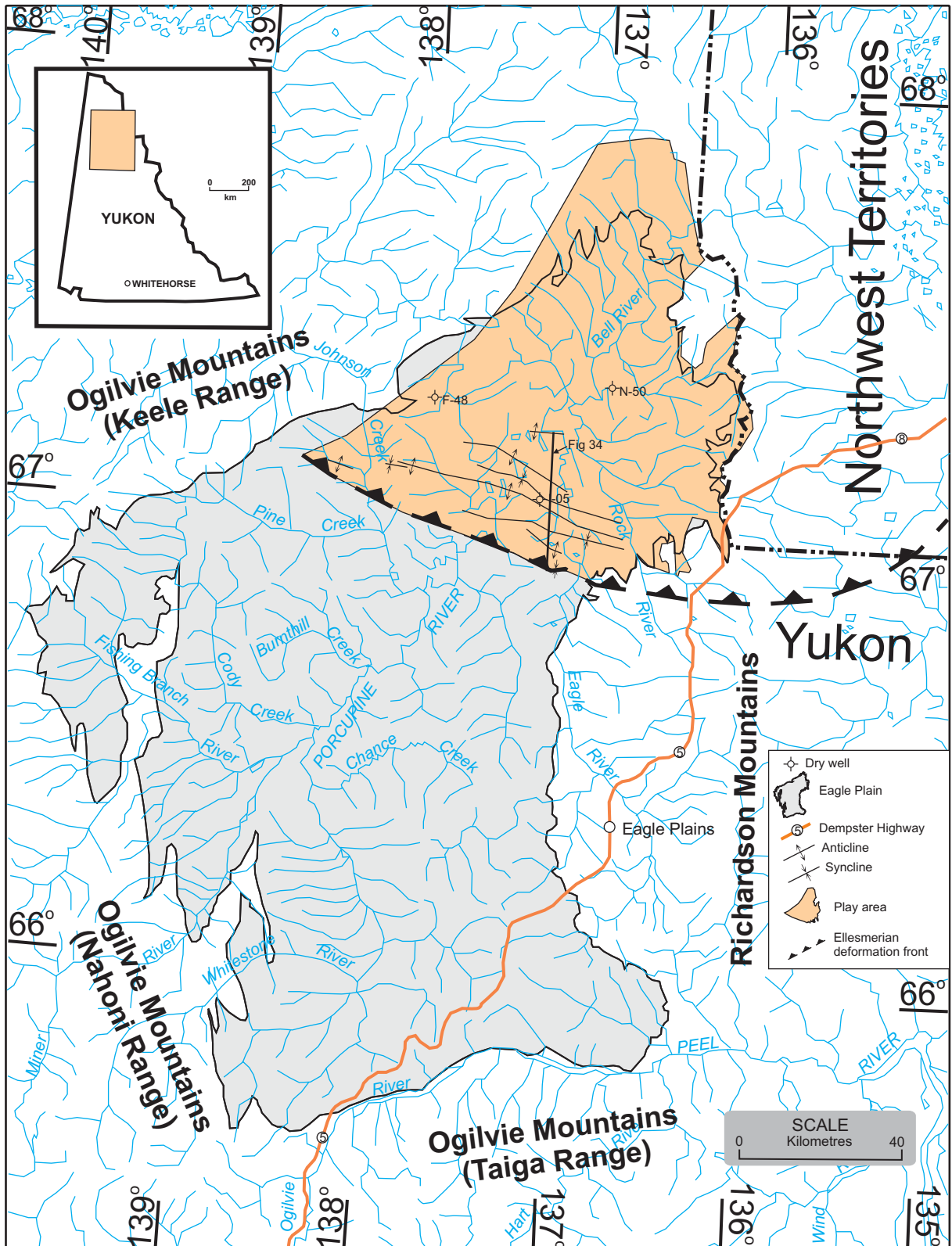
Figure 33. Imperial/Tuttle sandstone structural (Ellesmerian deformation-Bell Subbasin) oil and gas play. Interpreted Ellesmerian compressional structures (anticlines and synclines) and deformation front are depicted (from Lane (2007)). Seismic line location of Fig. 34 is shown.
