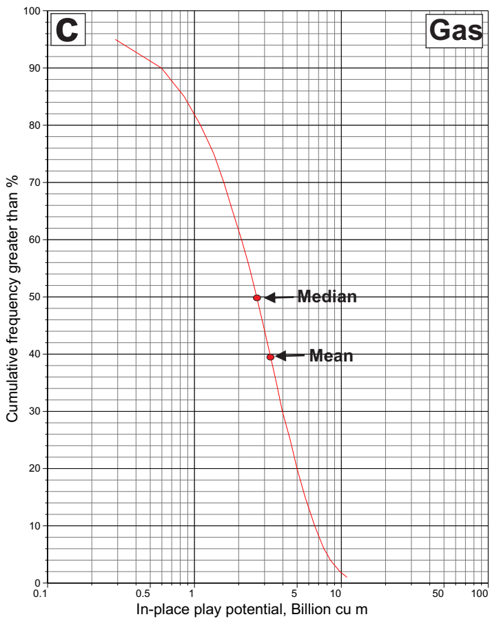
Figure 35. Estimates of in-place oil (a) and gas (c) potential of the Imperial/Tuttle sandstone structural (Ellesmerian deformation-Bell Subbasin) play. Pool-size-by-rank plots of the oil (b) and gas (d) plays are also displayed.
