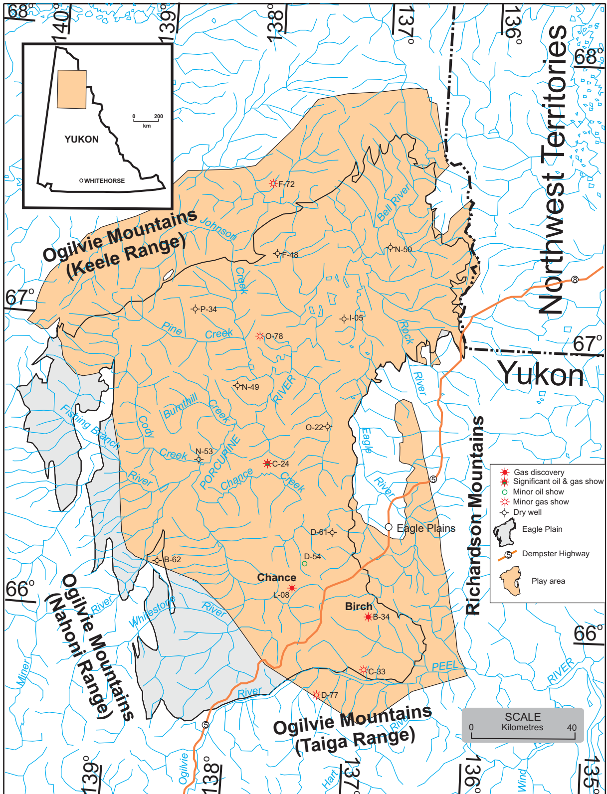
Figure 36. Imperial/Tuttle sandstone stratigraphic/combination oil and gas play.
