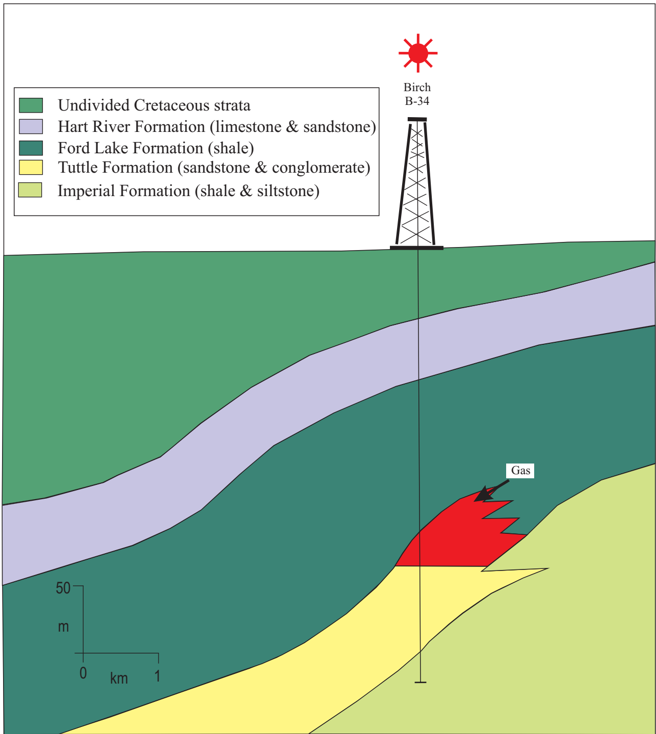
Figure 37. Schematic cross-section illustrating potential trap configurations in the Imperial/Tuttle sandstone stratigraphic/combination oil and gas play. Illustrated trap is an updip facies change where Tuttle porous sandstones abut against shale formations.. From National Energy Board, 2000.
